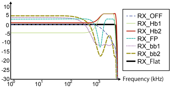
Receive Characteristics Curves
