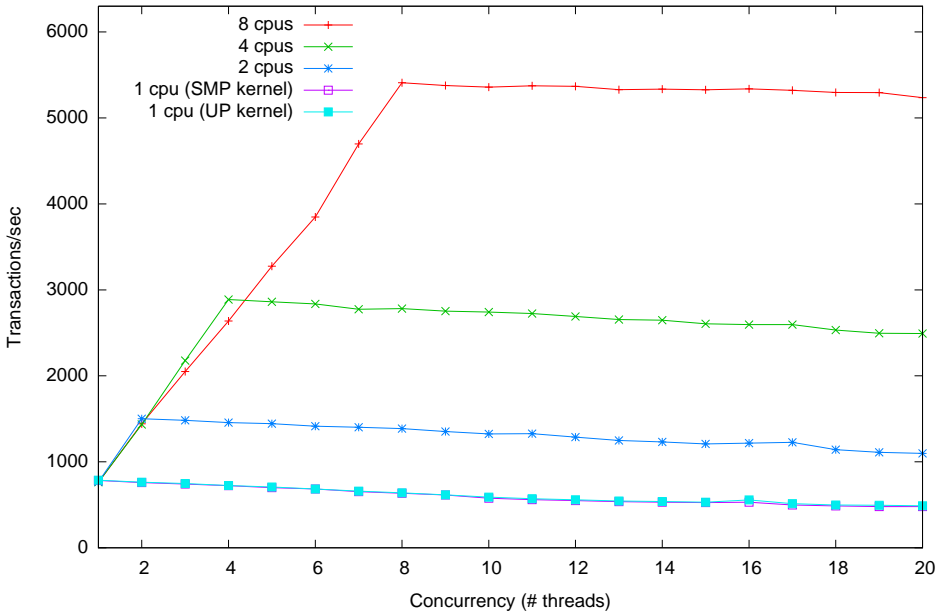
PostgreSQL sysbench on 8-core opteron, FreeBSD 7.0 with N CPUs active
