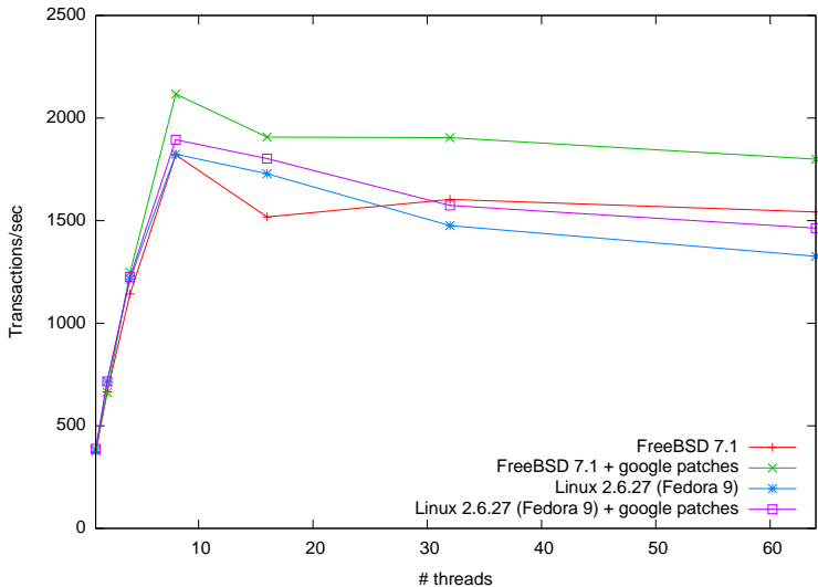
MySQL sysbench read-write performance on 8-core Xeon
