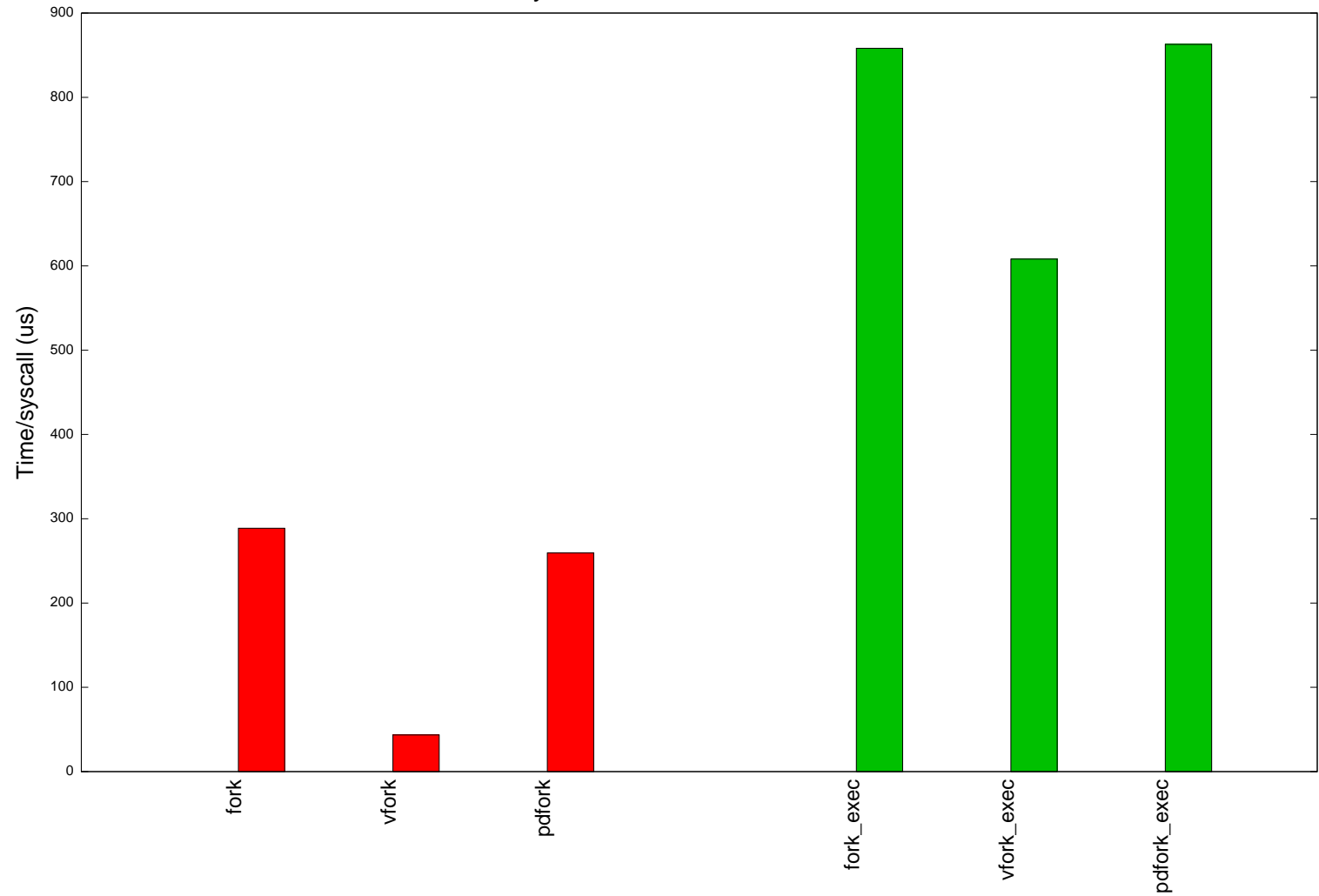
System call microbenchmarks
