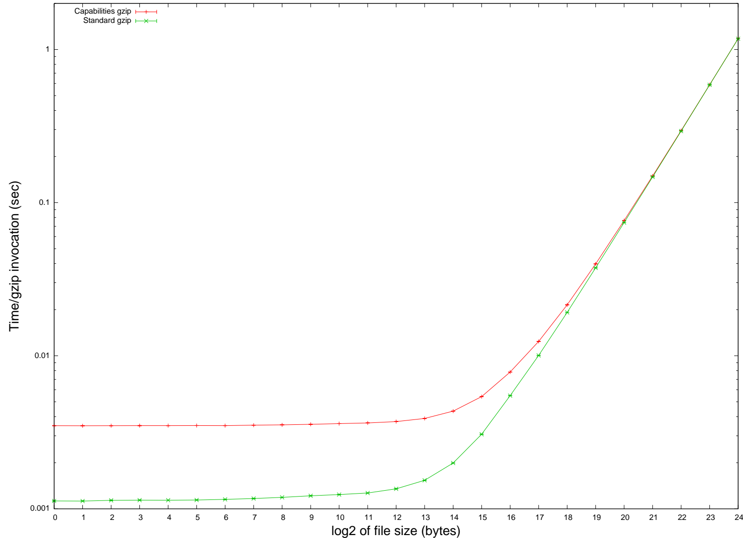
gzip run time with varying file sizes
