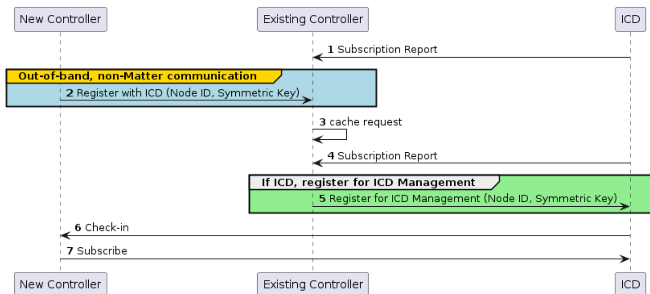
Figure 75. Infrastructure Assisted Proxy Registration
