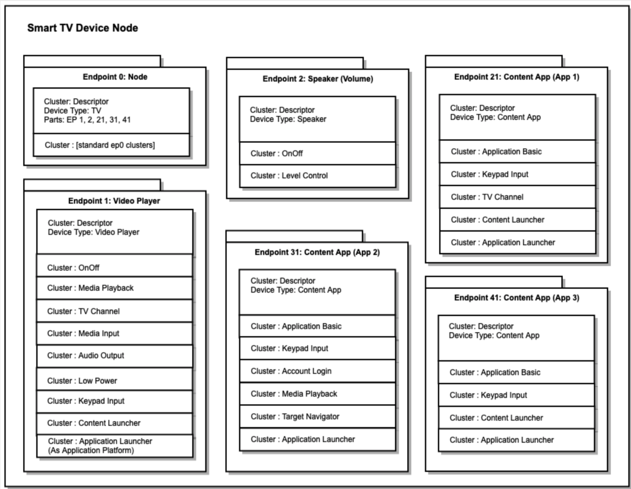
Figure 41. Endpoint Composition for Video Player Device
