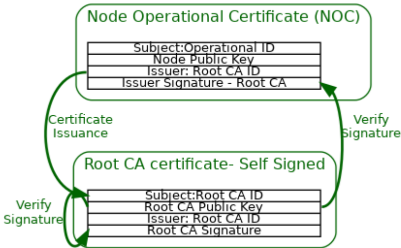
Figure 39. Node Operational Certificate PKI hierarchy without optional ICAC
