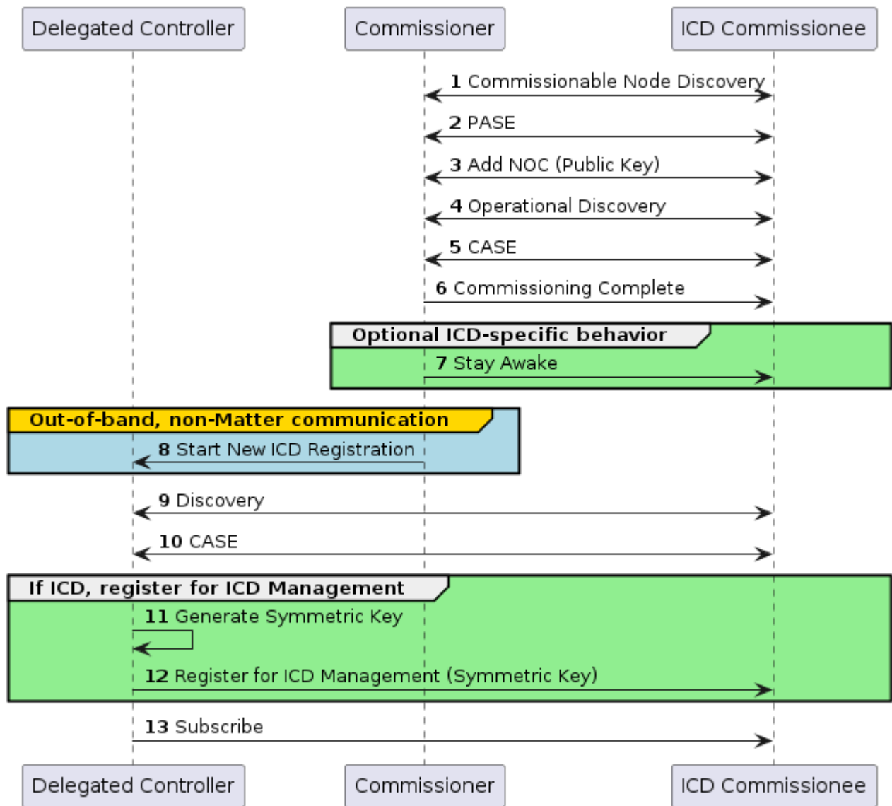
Figure 73. Delegated Controller Registration
