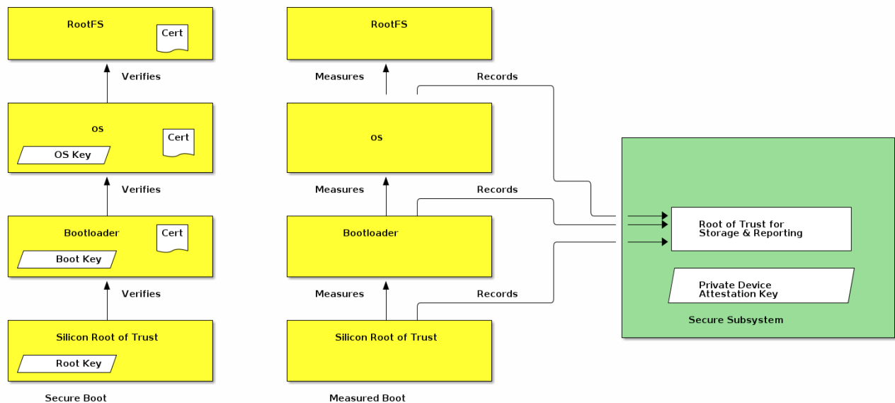
Figure 37. Illustration of the measured boot process
