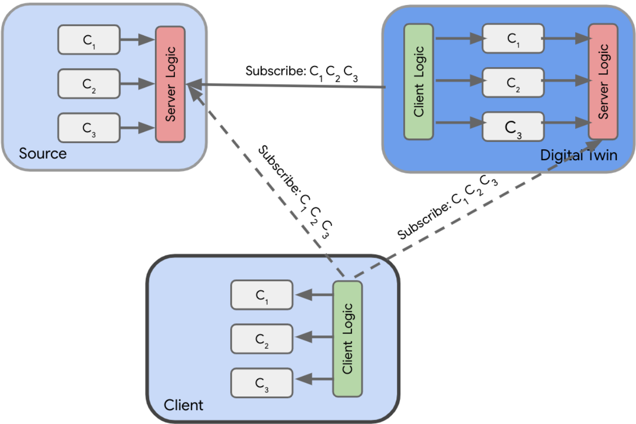
Figure 58. Digital twin acting as a proxy re-publishing clusters
