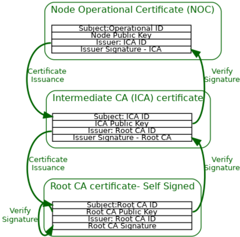
Figure 38. Node Operational Certificate PKI hierarchy with optional ICAC
