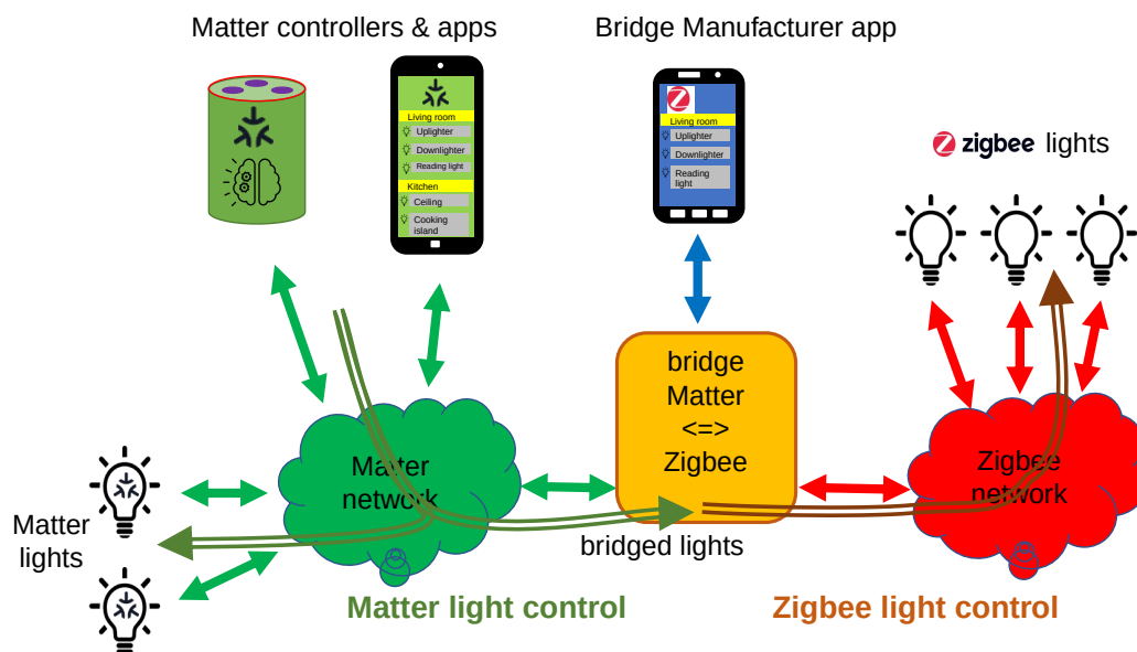
Figure 50. example of bridging lights
