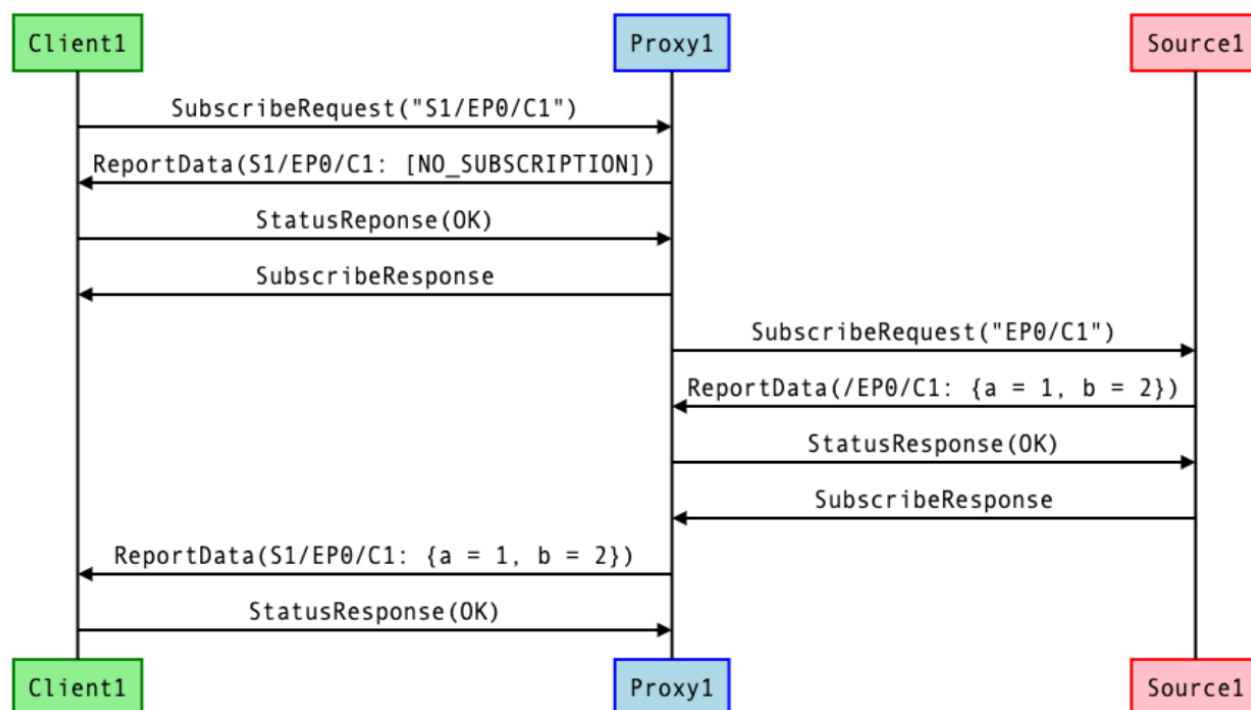
Figure 59. Upstream/Downstream subscription sequences
