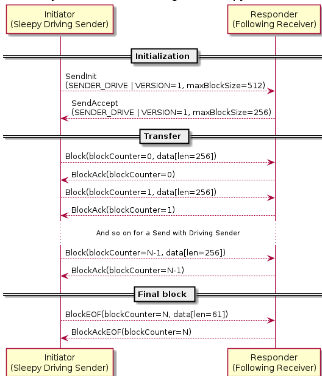
Figure 79. Synchronous file sending from sleepy device acting as driving Sender
