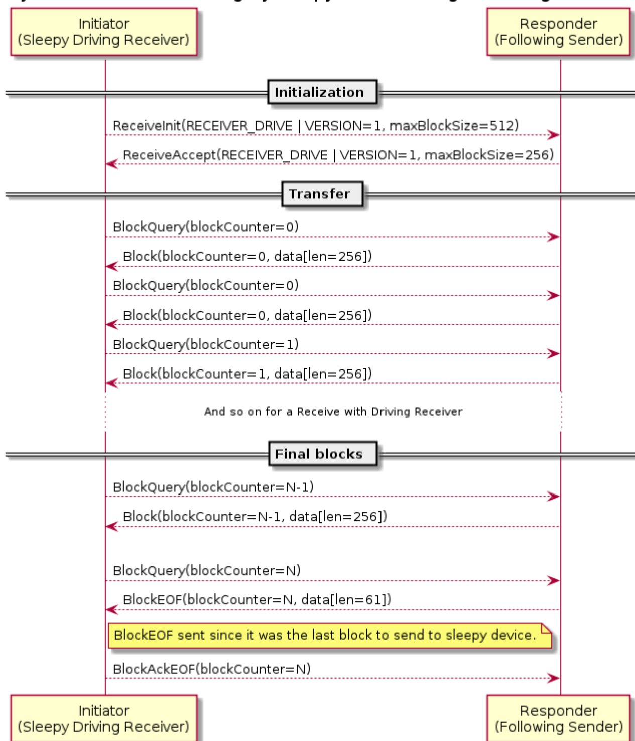
Figure 81. Synchronous file receiving by sleepy device acting as driving Receiver
