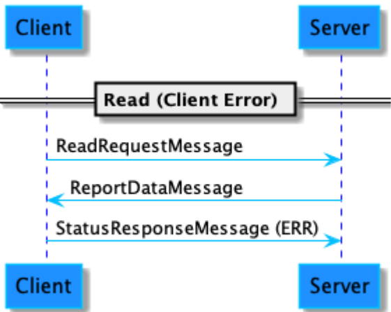
Figure 70. Read message with client-side error flow
