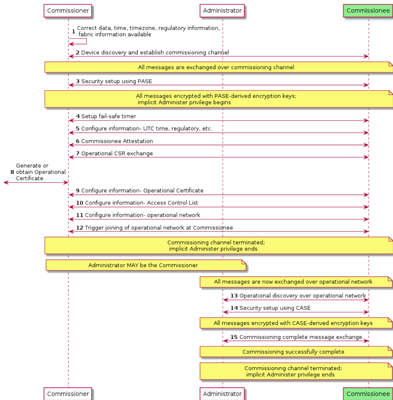
Figure 31. Non-concurrent connection commissioning flow
