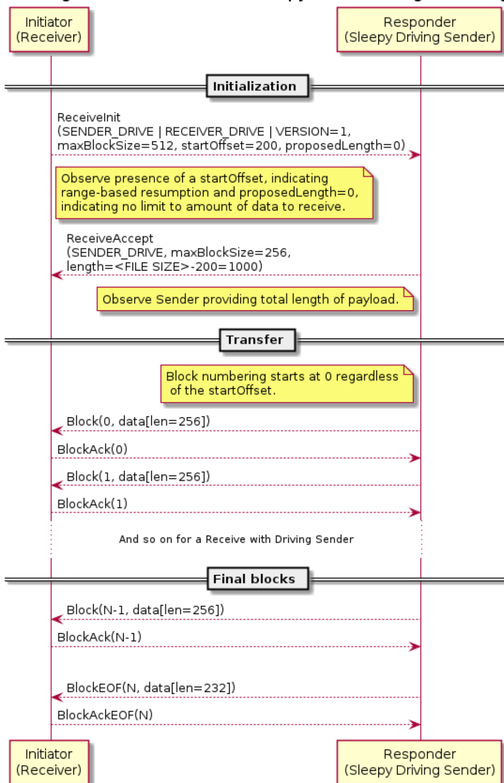
Figure 84. Re-started receive from sleepy device acting as driving Sender
