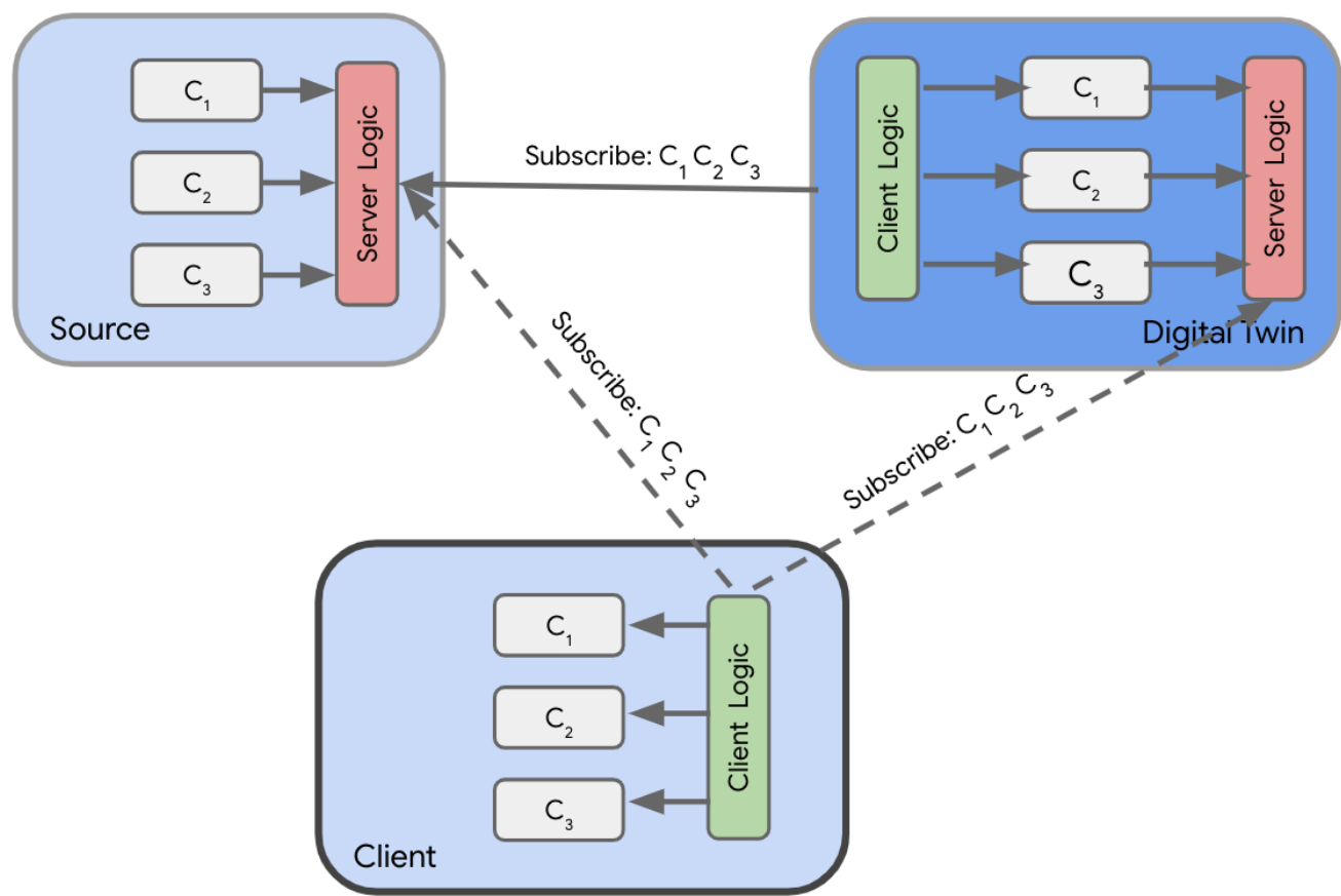
Figure 56. Digital twin acting as a proxy re-publishing clusters
