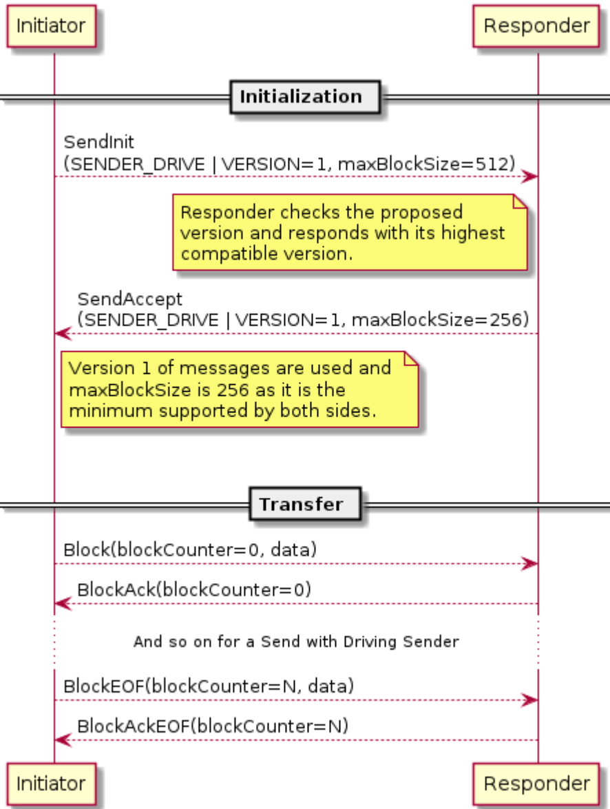
Figure 77. Version negotiation: both participants support V1 of the protocol
