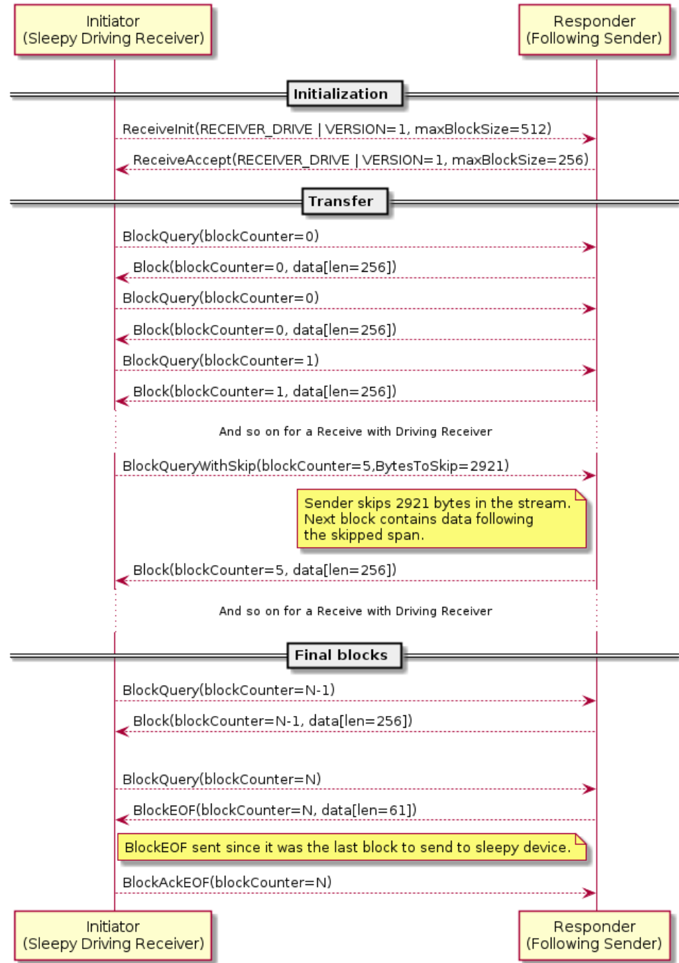
Figure 82. Synchronous file receiving by device acting as driving Receiver, including BlockQueryWithSkip
