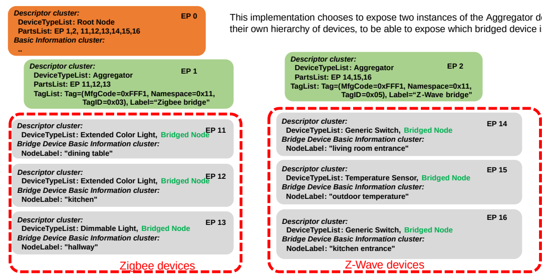
Figure 44. example of endpoints representing Bridged Devices from two technologies
