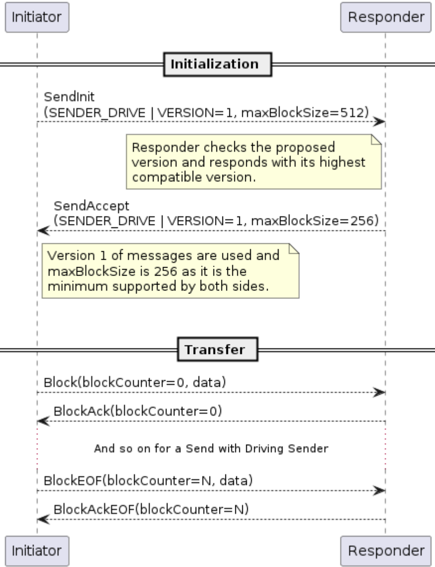
Figure 90. Version negotiation: both participants support V1 of the protocol
