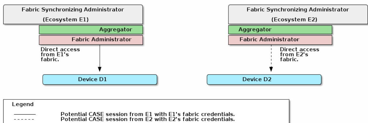
Figure 105. Fabric Synchronization Setup - Example Starting Condition.
