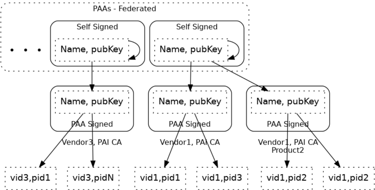
Figure 39. Device Attestation PKI hierarchy
