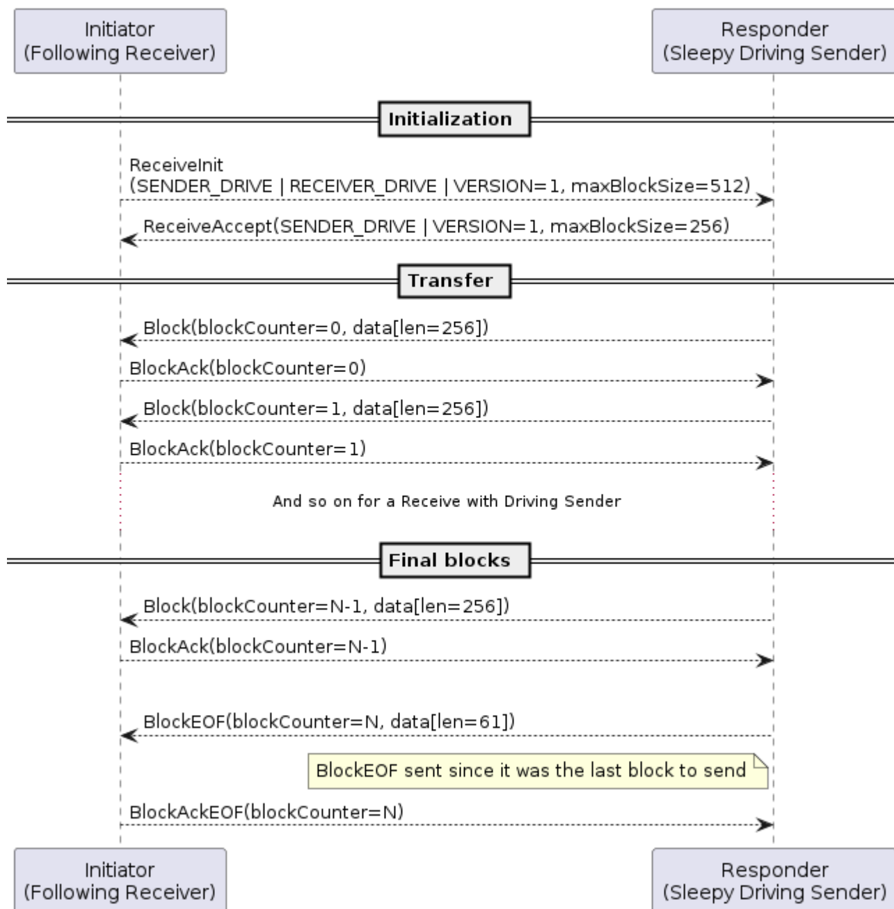
Figure 96. Synchronous file receive from sleepy device acting as driving Sender
