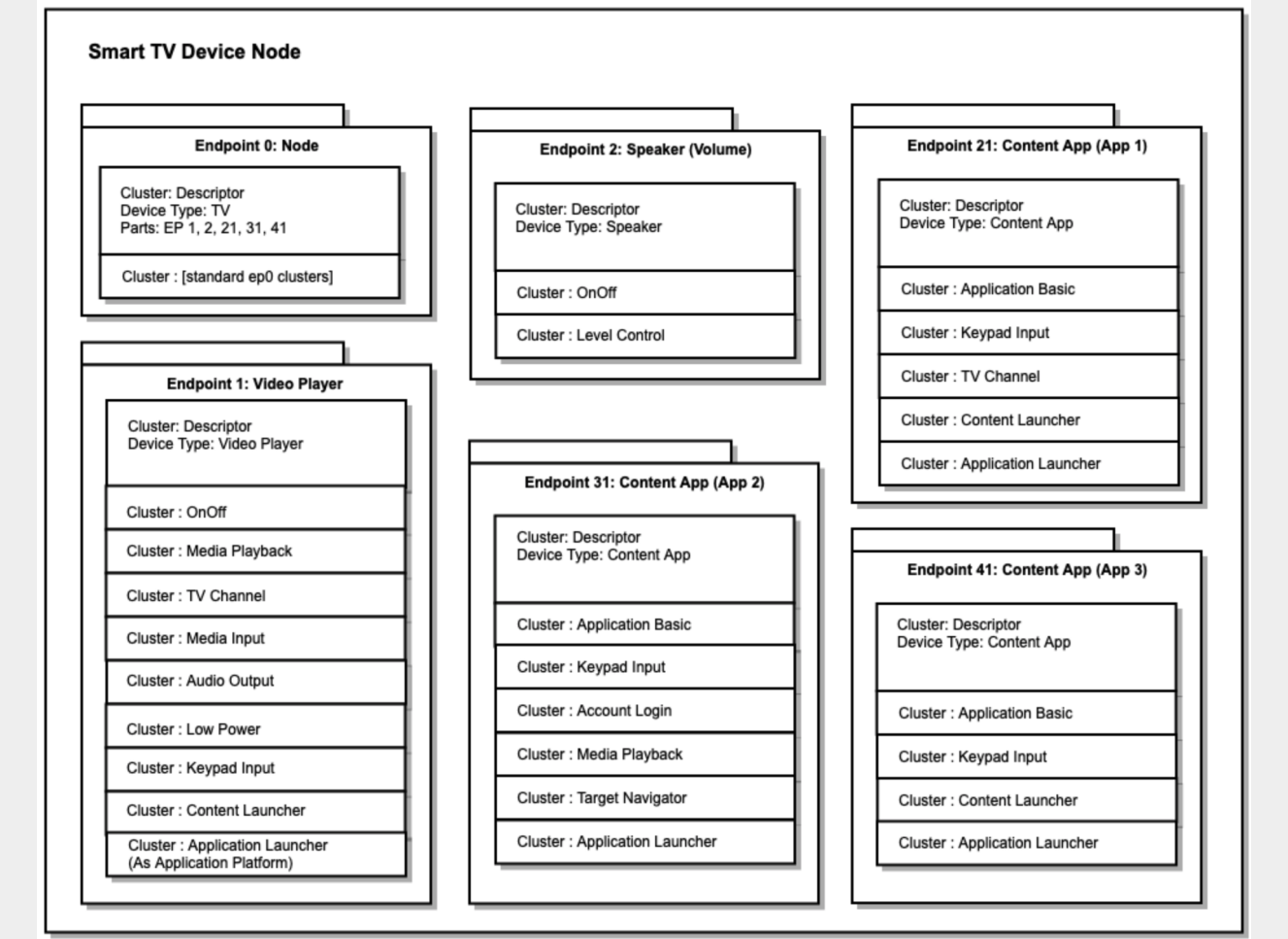
Figure 44. Endpoint Composition for Video Player Device
