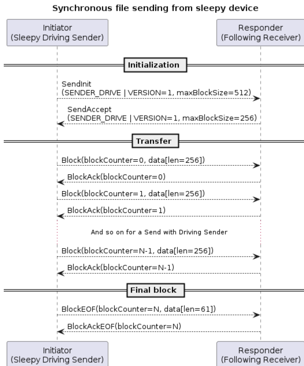
Figure 92. Synchronous file sending from sleepy device acting as driving Sender
