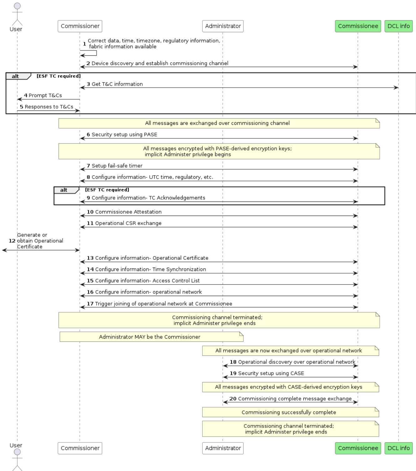
Figure 33. Non-concurrent connection commissioning flow
