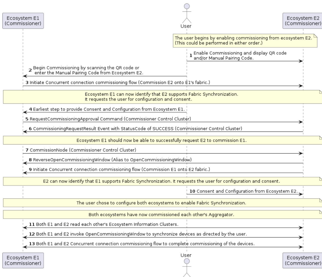
Figure 110. Fabric Synchronization Setup - Example Complete Flow.
