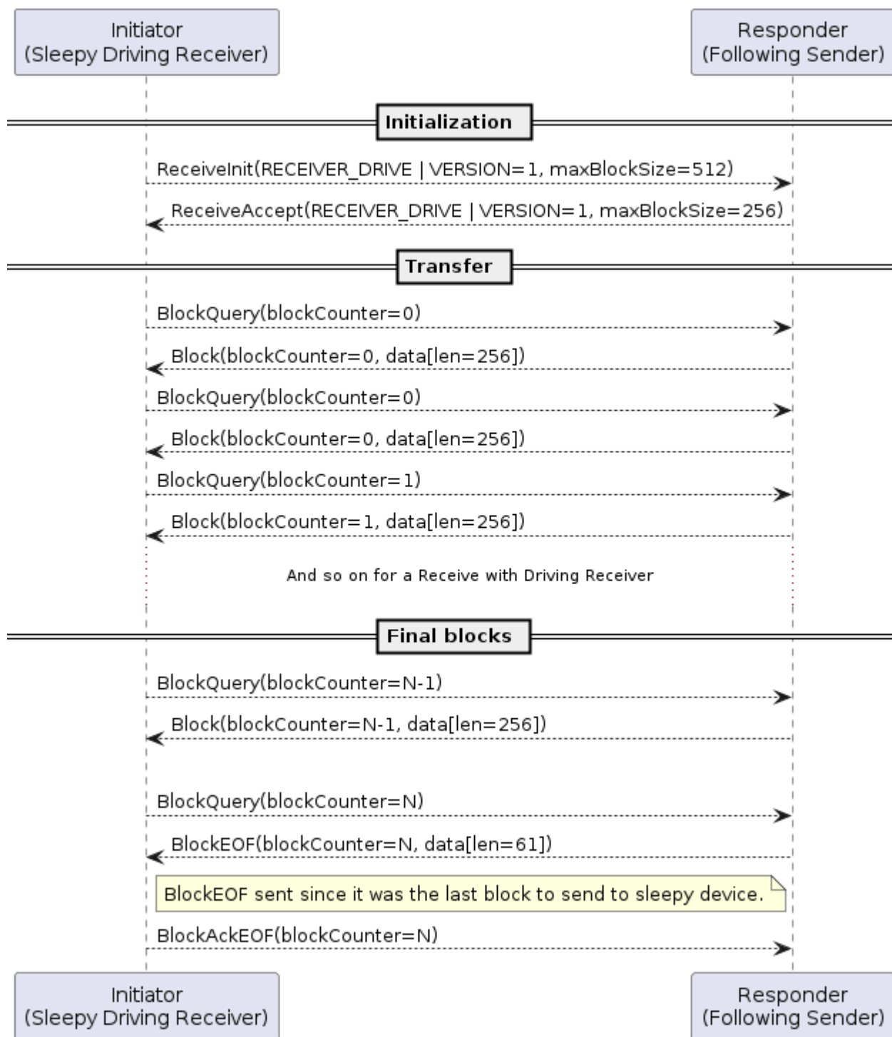
Figure 94. Synchronous file receiving by sleepy device acting as driving Receiver
