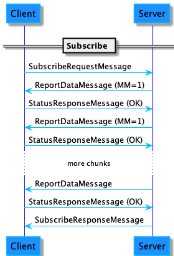
Figure 86. Subscription flow
