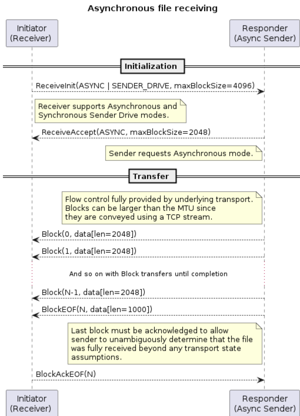
Figure 100. Asynchronous file receiving
