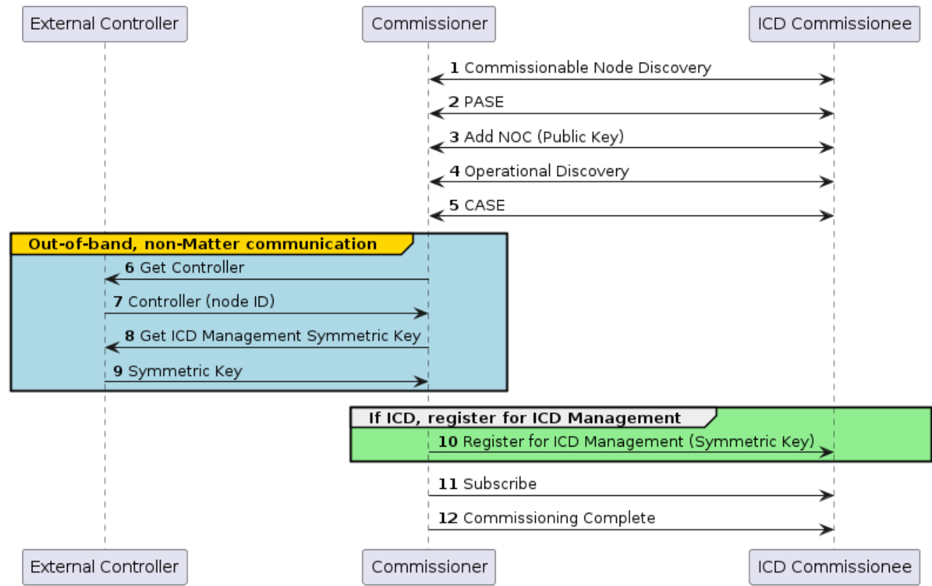
Figure 77. External Controller Registration
