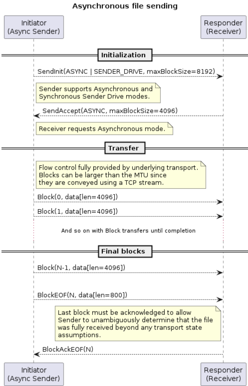
Figure 99. Asynchronous file sending
