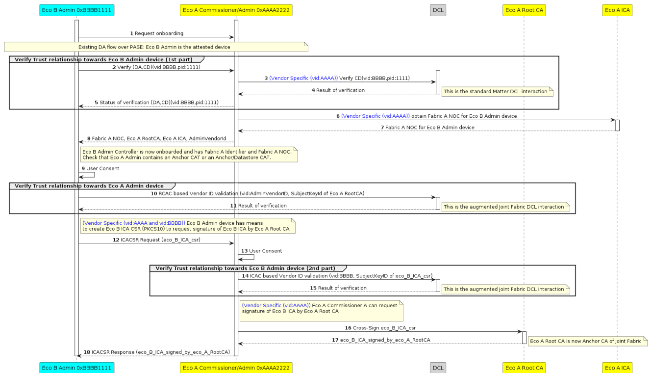
Figure 102. Joint Commissioning Steps
