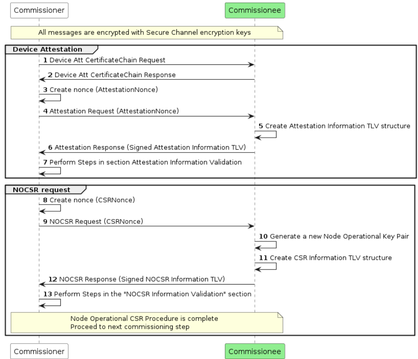
Figure 43. Node Operational Credentials flow
