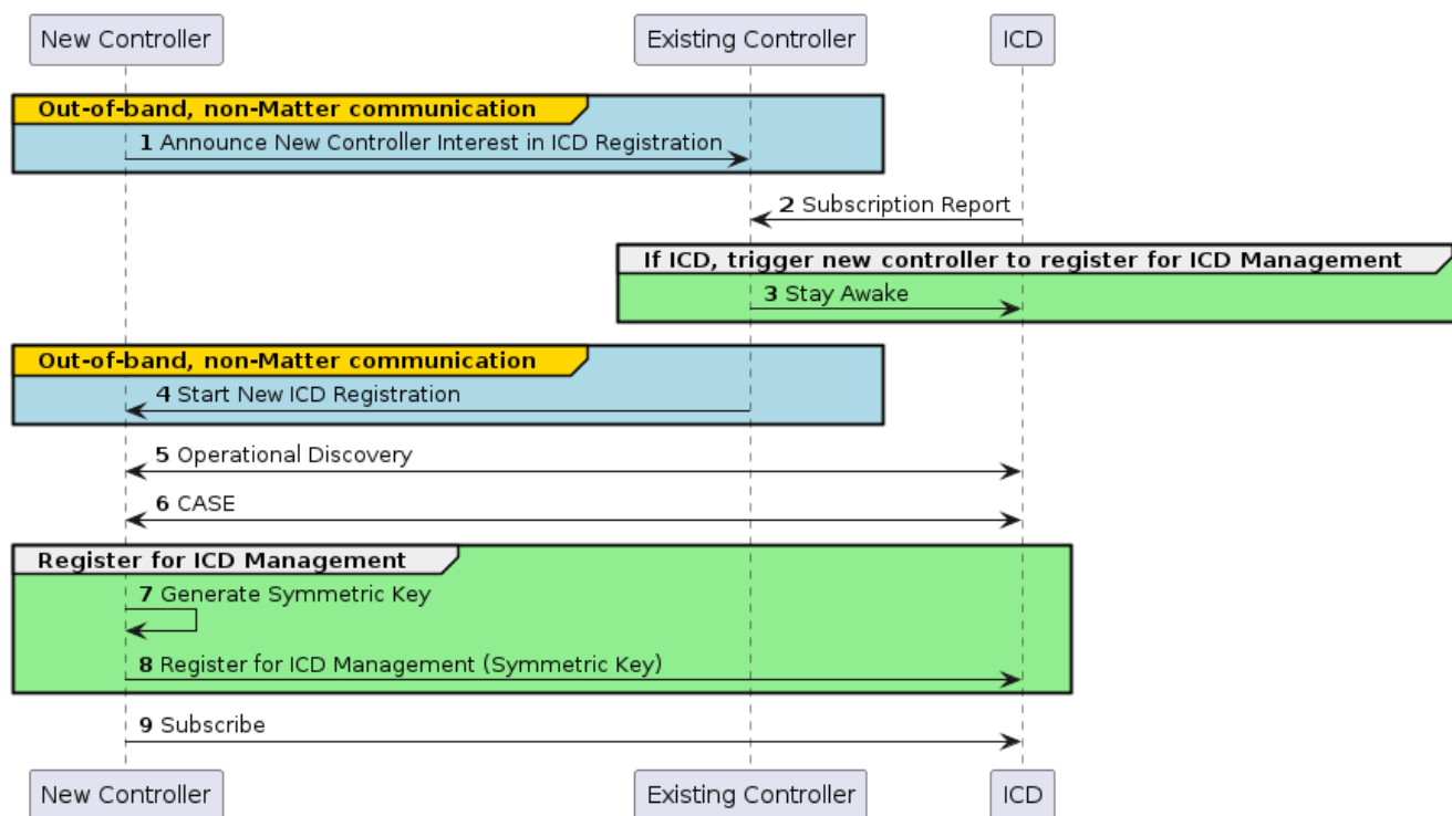
Figure 79. Infrastructure Assisted On-Demand Registration
