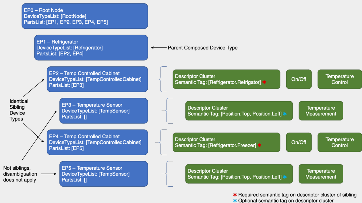
Figure 45. Disambiguation and information via semantic tags
