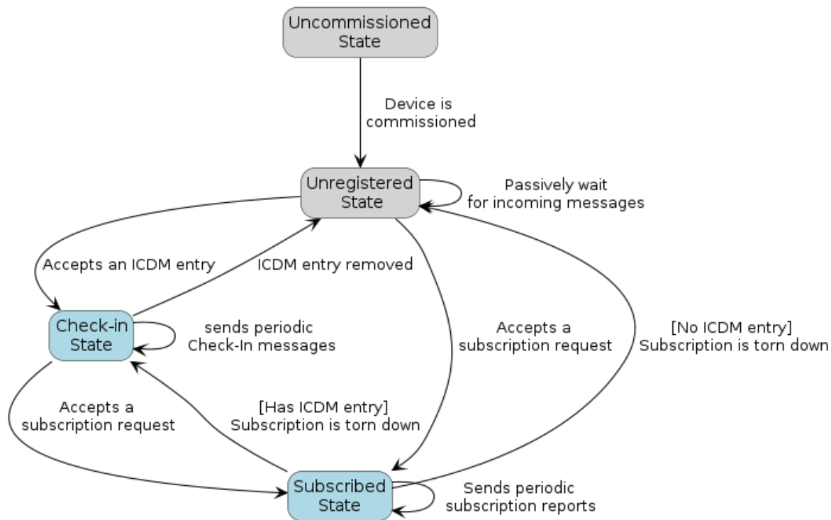
Figure 73. ICD State Machine
