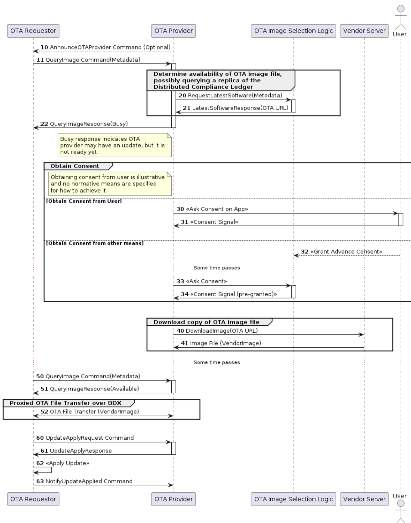
Figure 89. Detailed OTA Software Update Workflow
