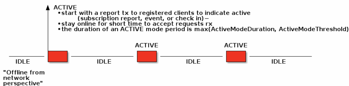
Figure 74. ICD Steady State Behavior Diagram
