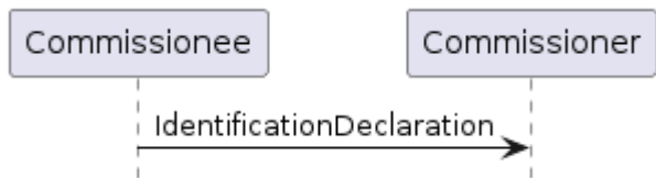
Figure 30. Overview of the UDC Protocol Identification Declaration message
