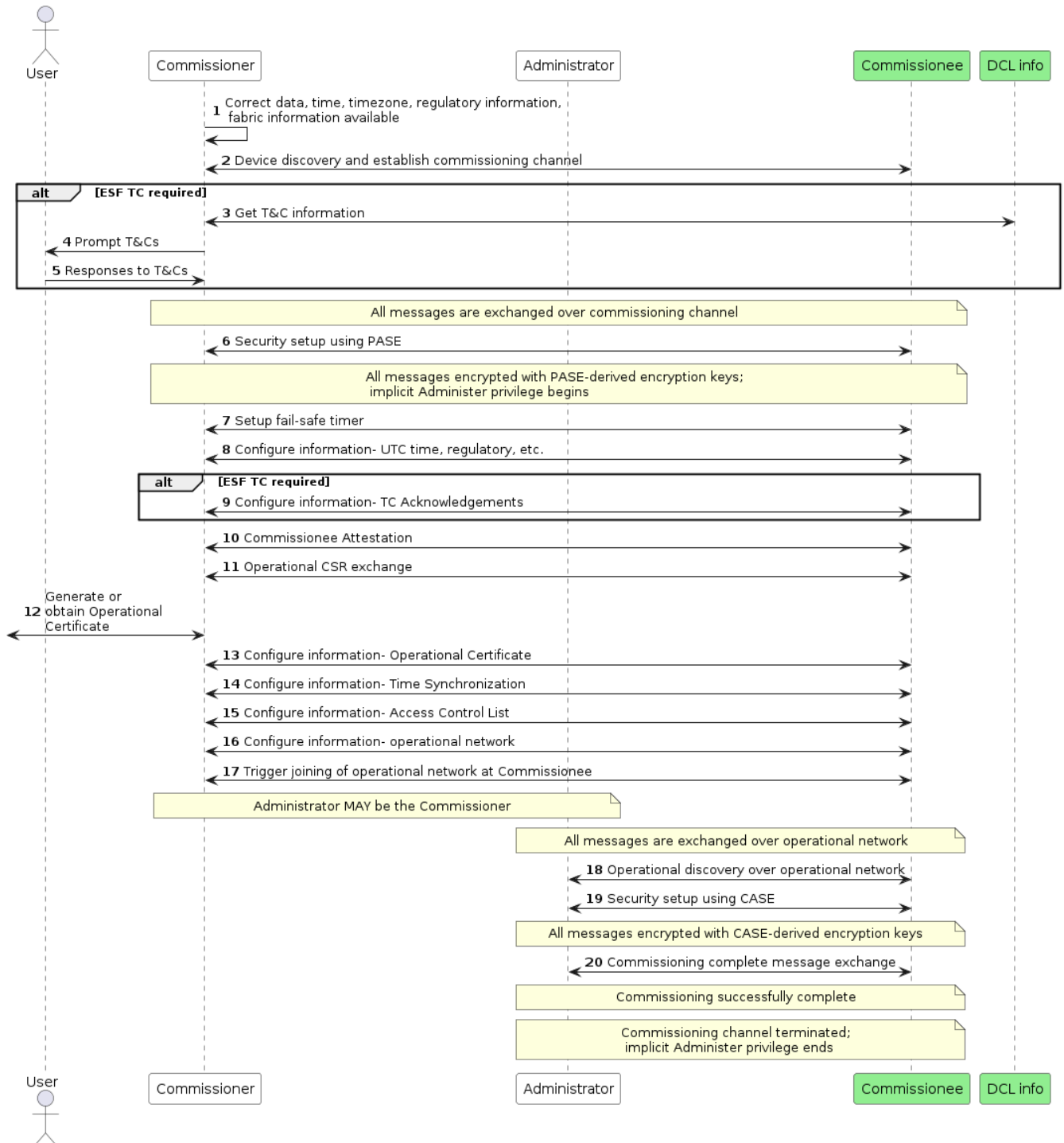
Figure 32. Concurrent connection commissioning flow
