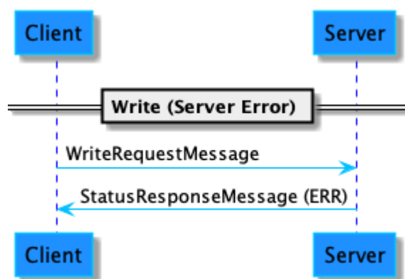
Figure 85. Write message with server-side error flow
