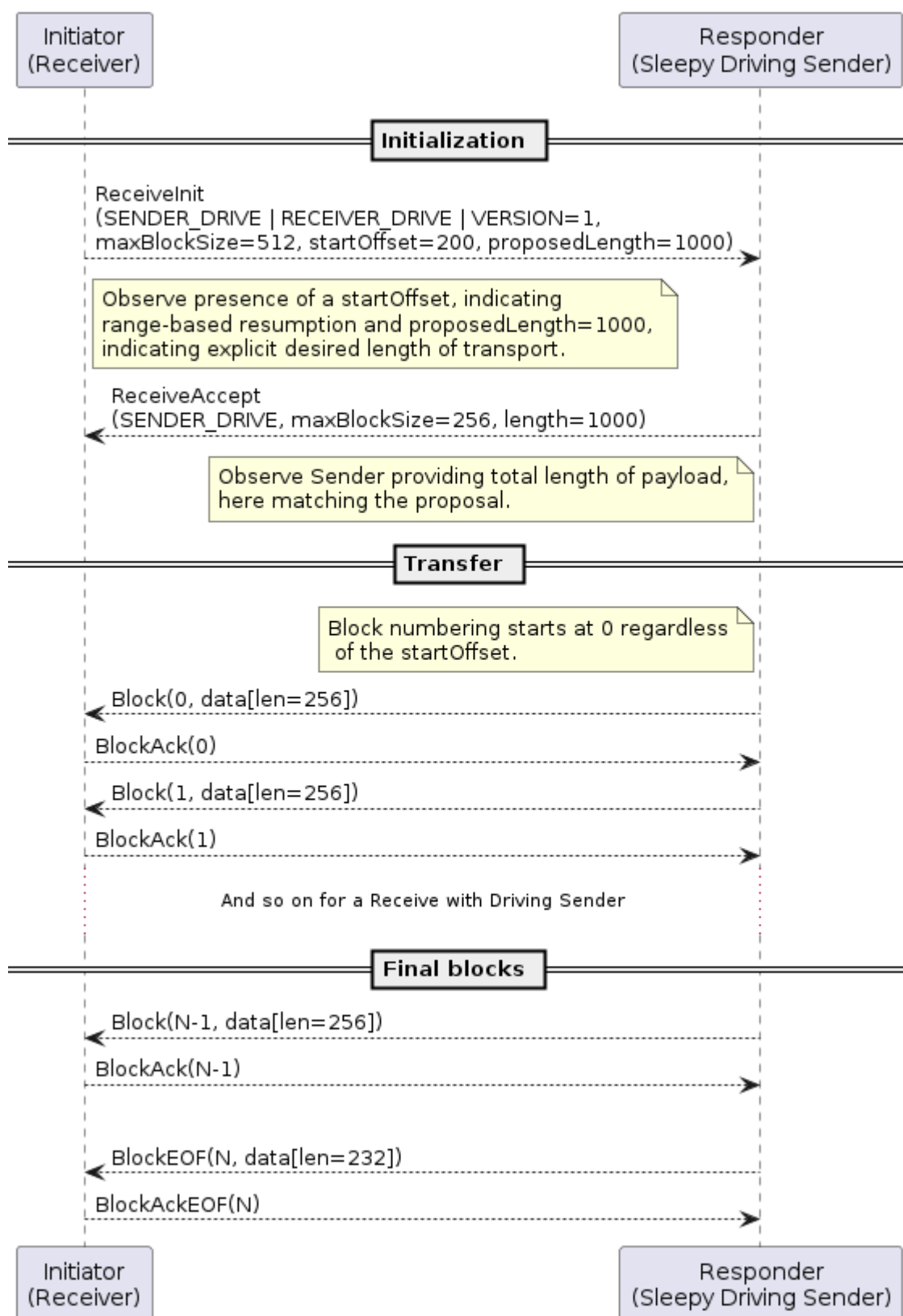
Figure 98. Range-based receive from sleepy device acting as driving Sender
