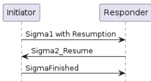
Figure 16. Session Resumption
