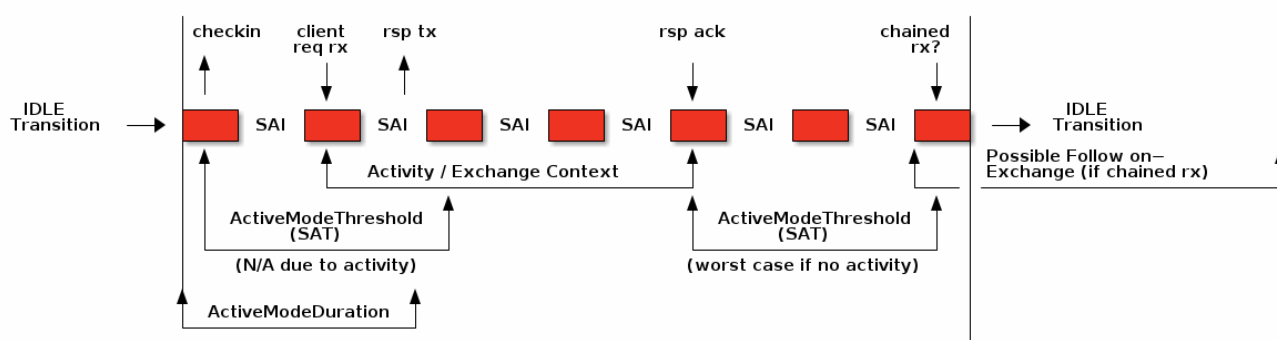
Figure 75. ICD Active Mode Behavior Diagram
