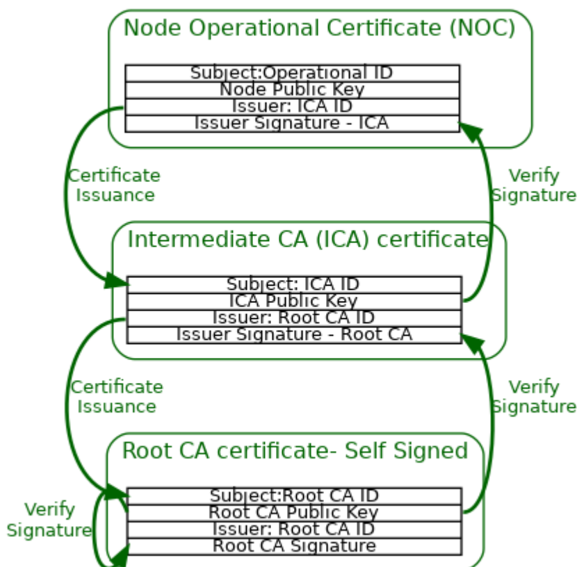
Figure 41. Node Operational Certificate PKI hierarchy with optional ICAC
