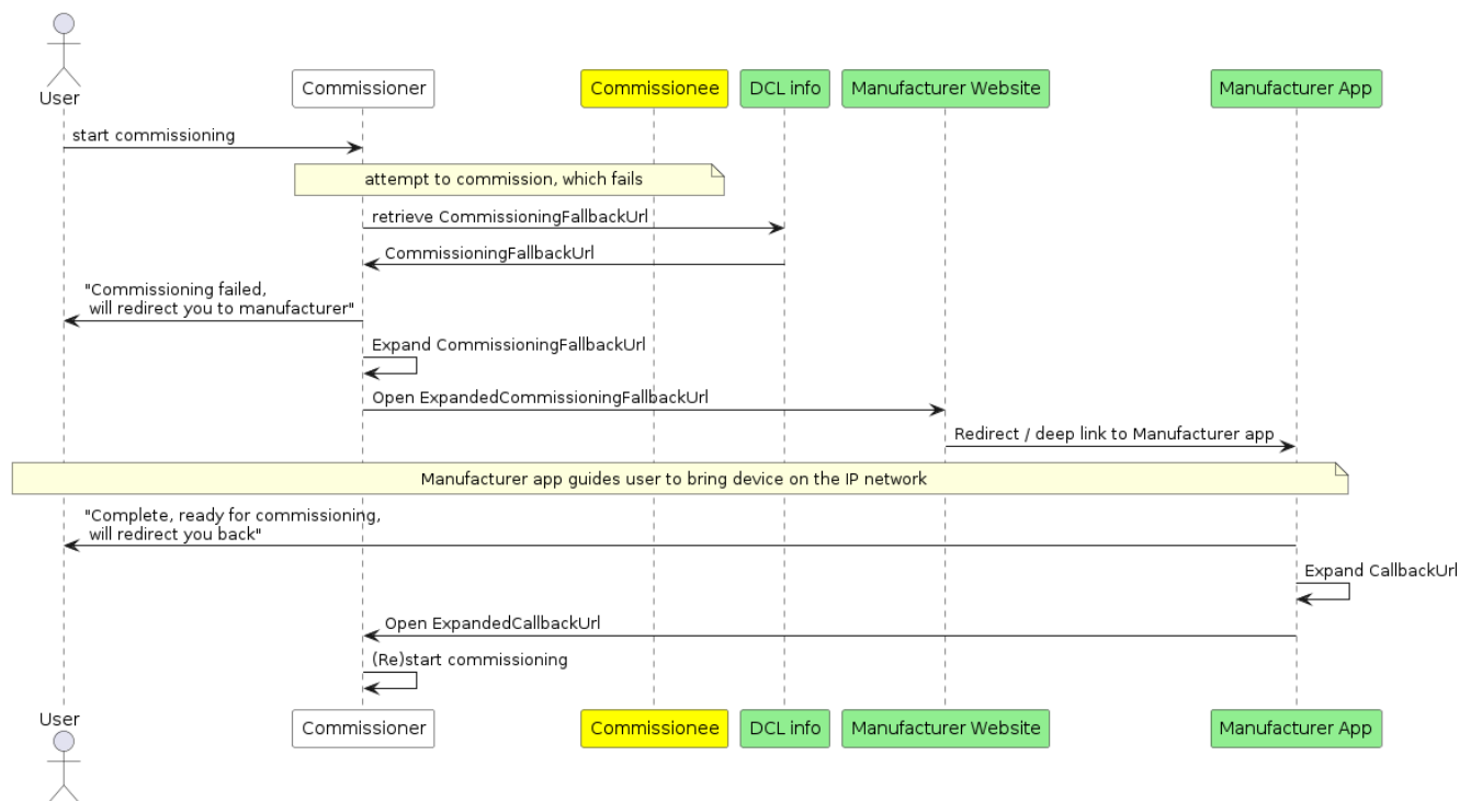
Figure 38. Commissioning Fallback Mechanism sequence diagram
