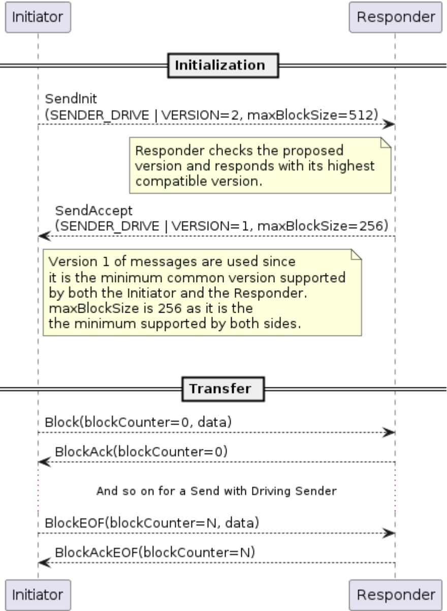
Figure 91. Version negotiation: Initiator supports V2 of the protocol, while Responder supports V1
