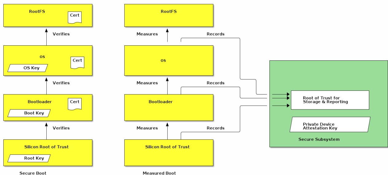
Figure 40. Illustration of the measured boot process
