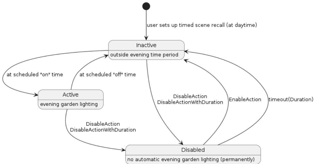
Figure 59. State diagram for example 'scheduled scene recall'
