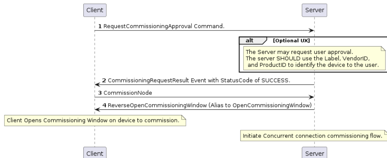
Figure 101. Commissioner Control Cluster - General Flow
