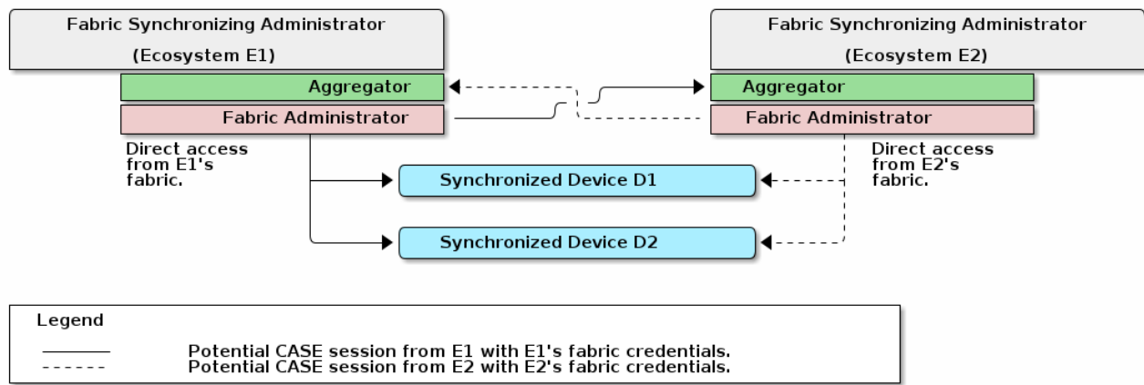
Figure 109. Fabric Synchronization Setup - Setup Complete.
