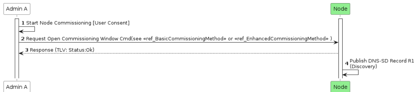
Figure 34. Open Commissioning Window (Administrator A)
