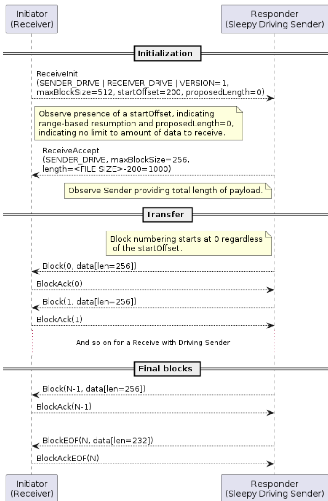
Figure 97. Re-started receive from sleepy device acting as driving Sender
