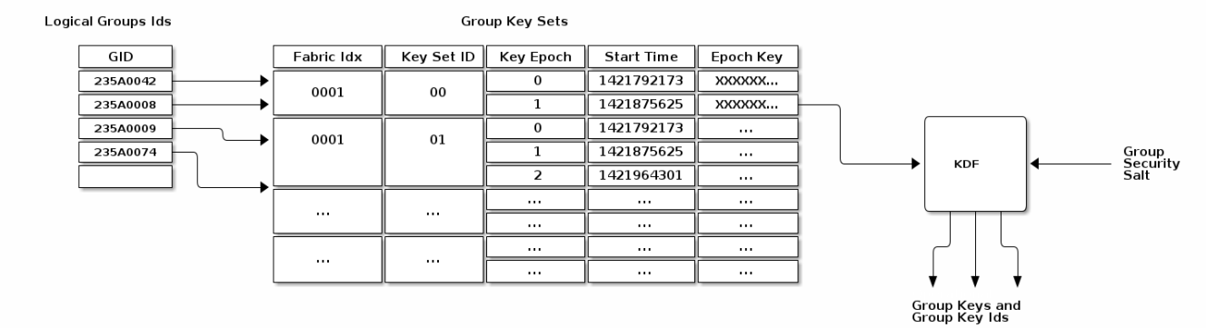
Figure 17. Group Key Derivation
