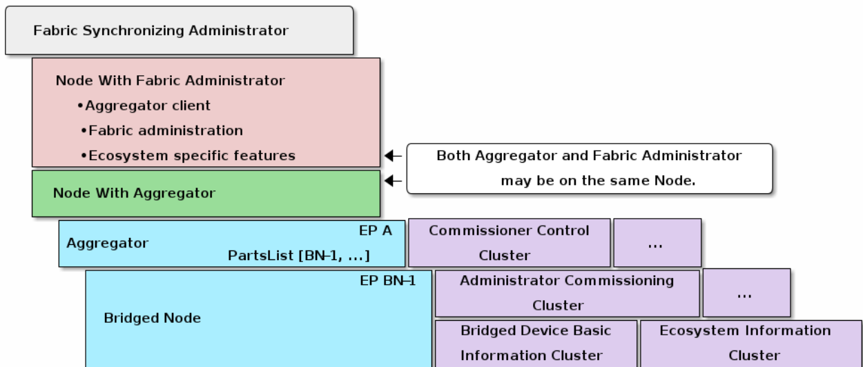
Figure 104. Composition of a device supporting Fabric Synchronization.
