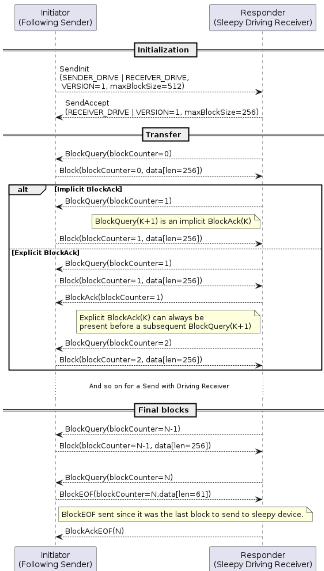
Figure 93. Synchronous file sending to sleepy device acting as driving Receiver
