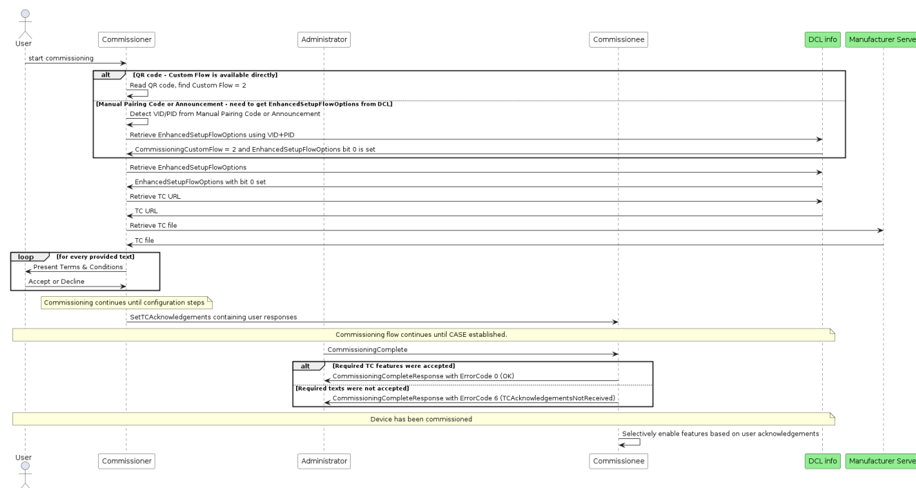
Figure 36. Enhanced Setup Flow TC commissioning sequence diagram
