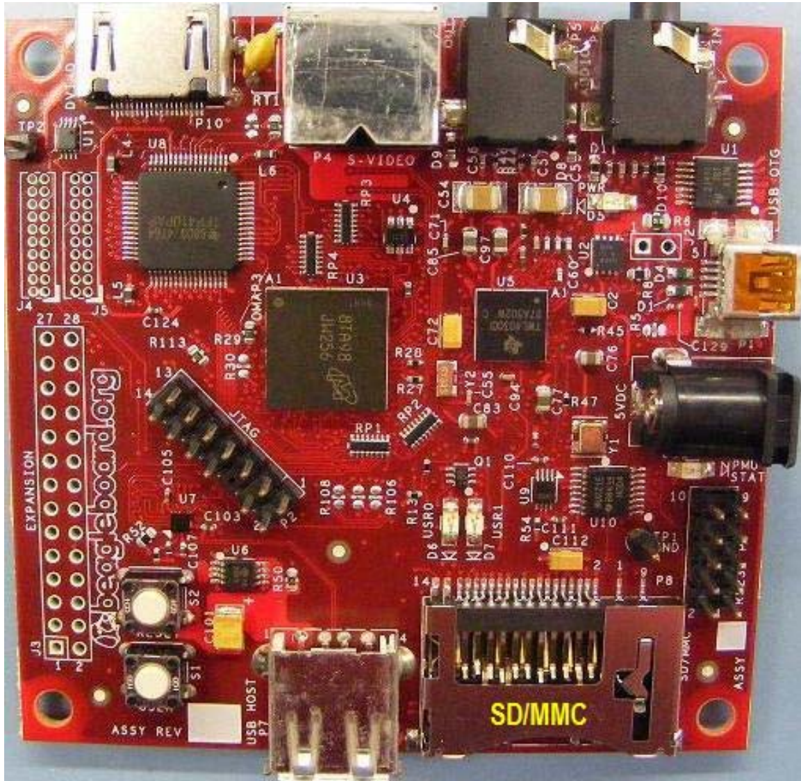
Figure 16. BeagleBoard SD/MMC Location
