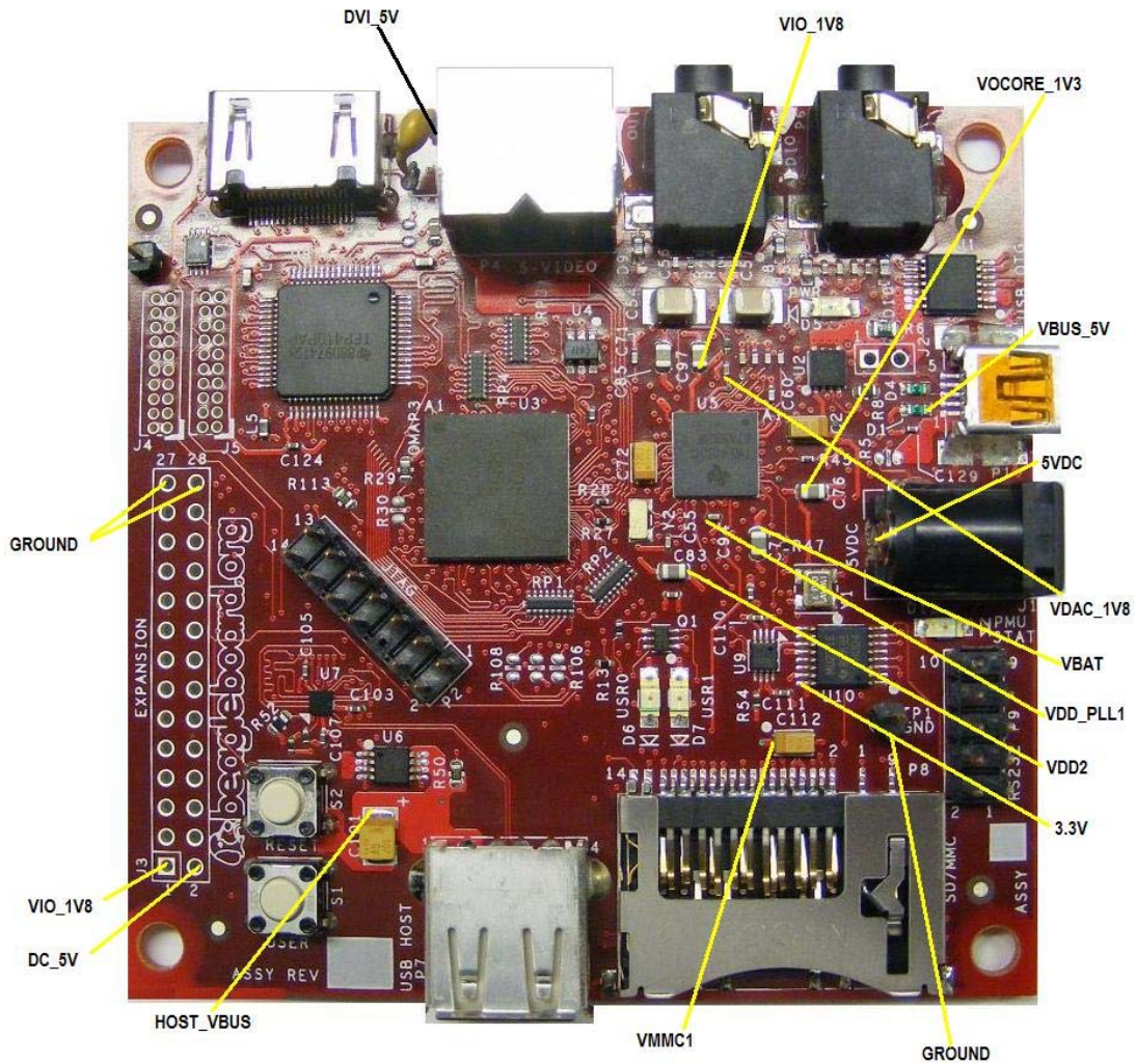
Figure 79. BeagleBoard Voltage Access Points
