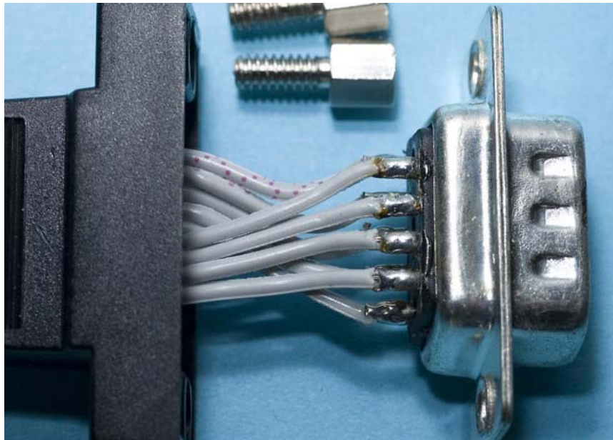
Figure 68. RS232 Cable
