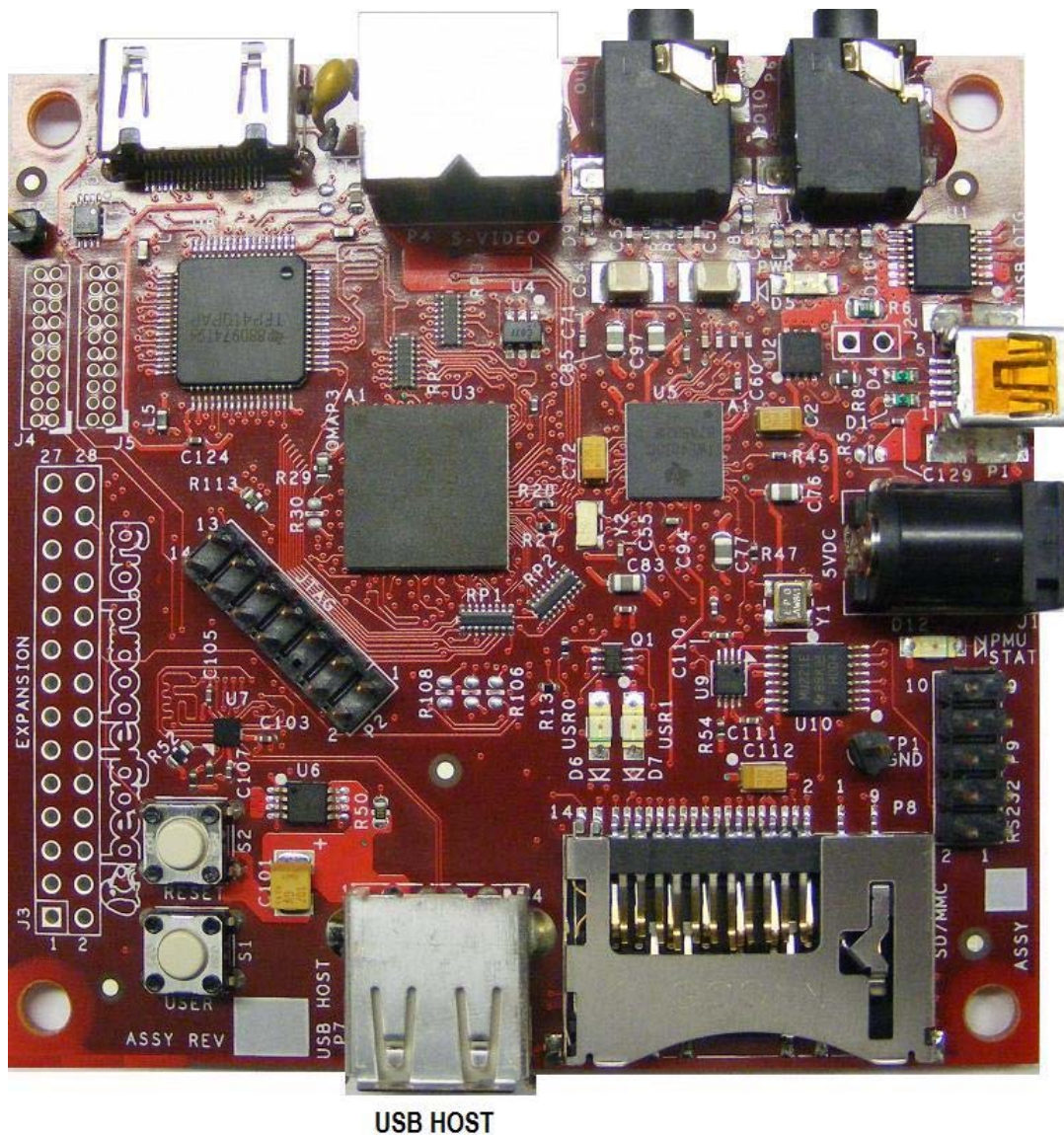
Figure 6. USB Host Connection
