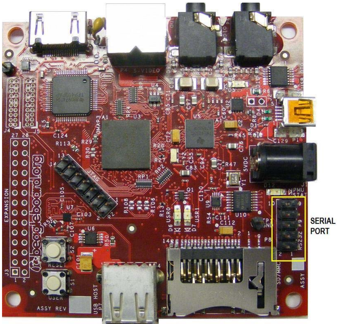
Figure 9. BeagleBoard Serial Cable Connection
