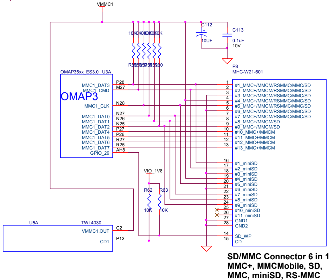
Figure 38. SD/MMC Interface
