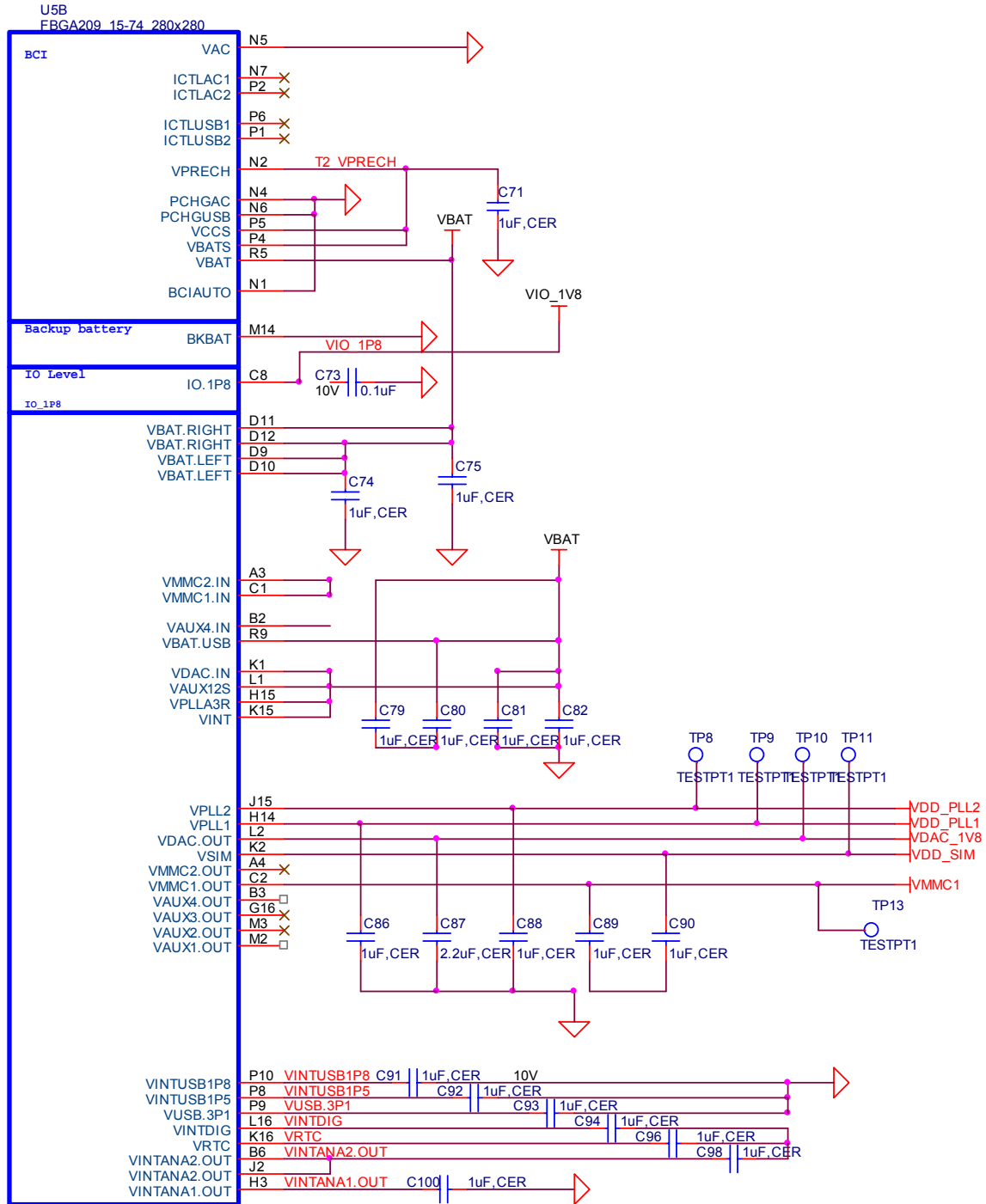
Figure 25. Peripheral Voltages
