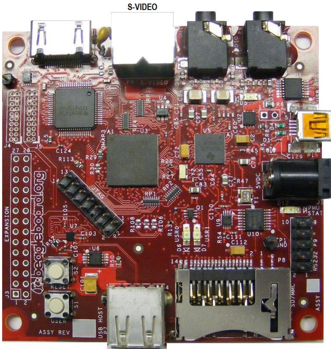
Figure 10. BeagleBoard S-Video Connection
