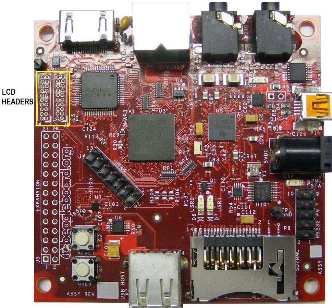
Figure 17. BeagleBoard LCD Header Location
