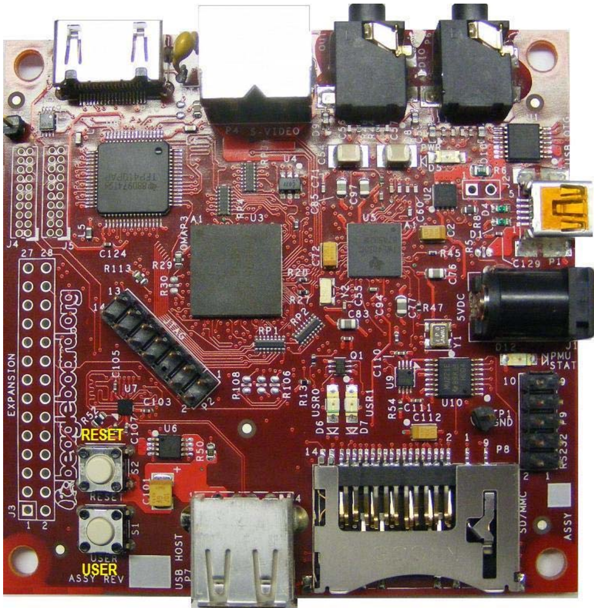
Figure 15. BeagleBoard Button Location
