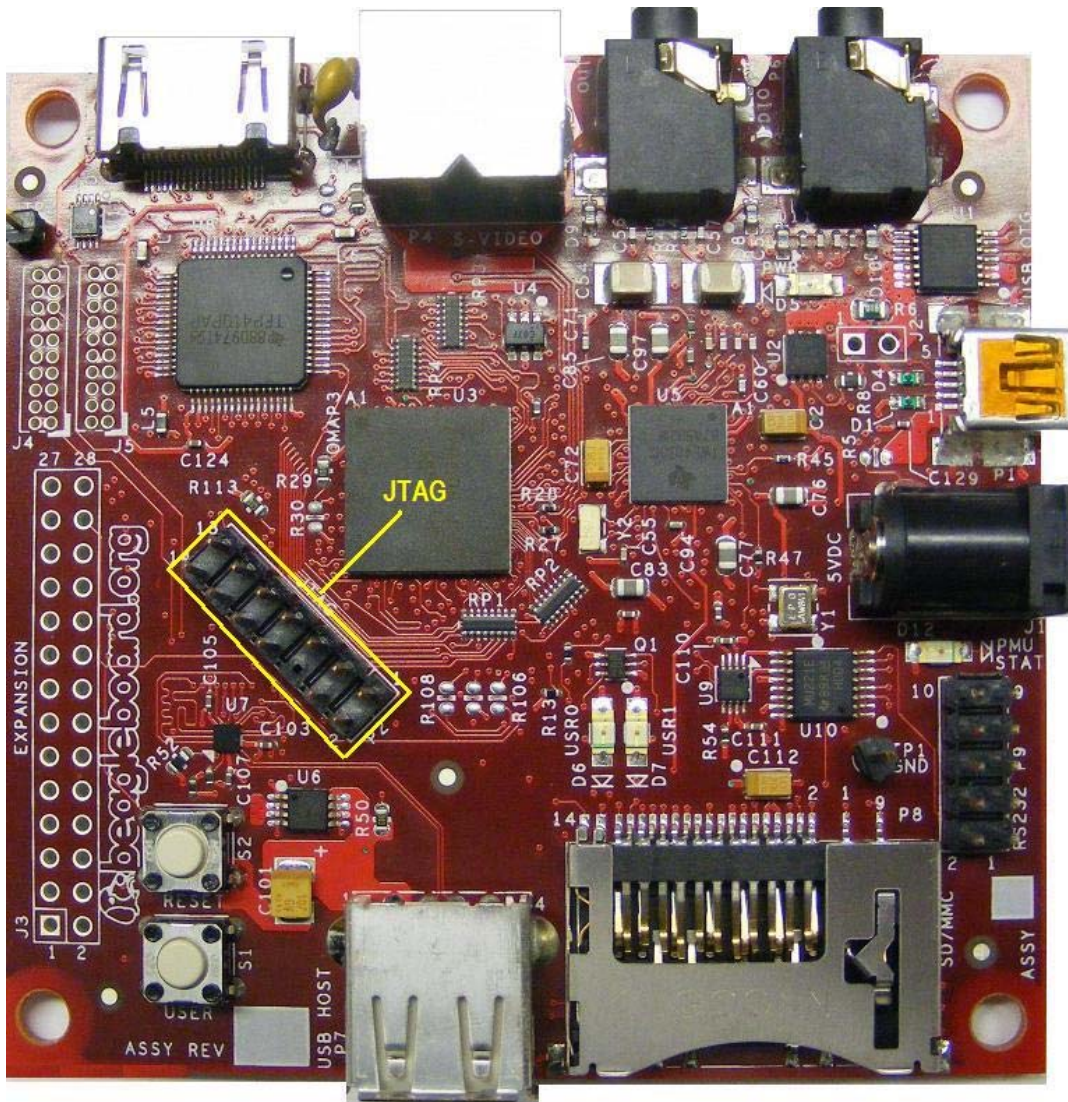
Figure 8. BeagleBoard JTAG Connection
