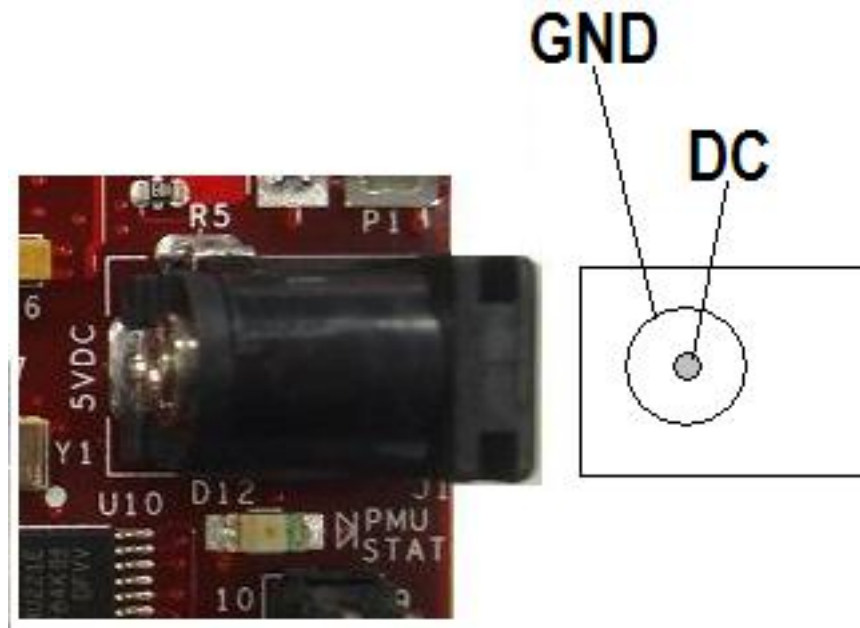
Figure 47. Power Connector
