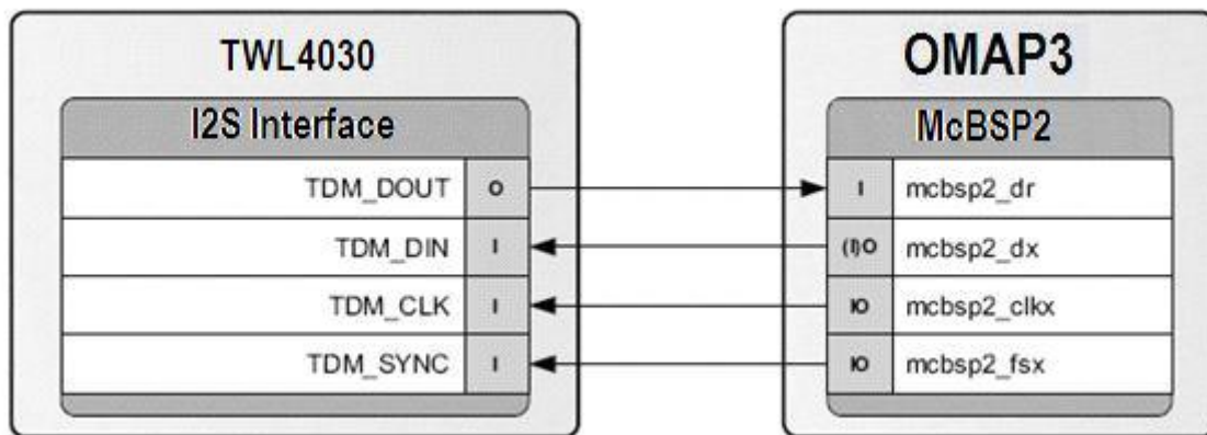
Figure 29. McBSP2 Interface
