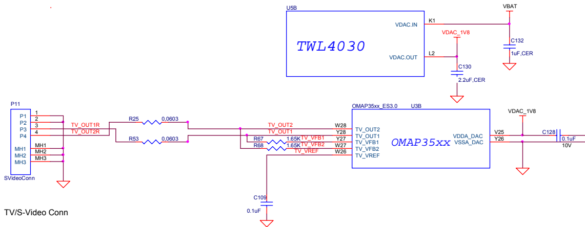
Figure 41. S-Video Interface
