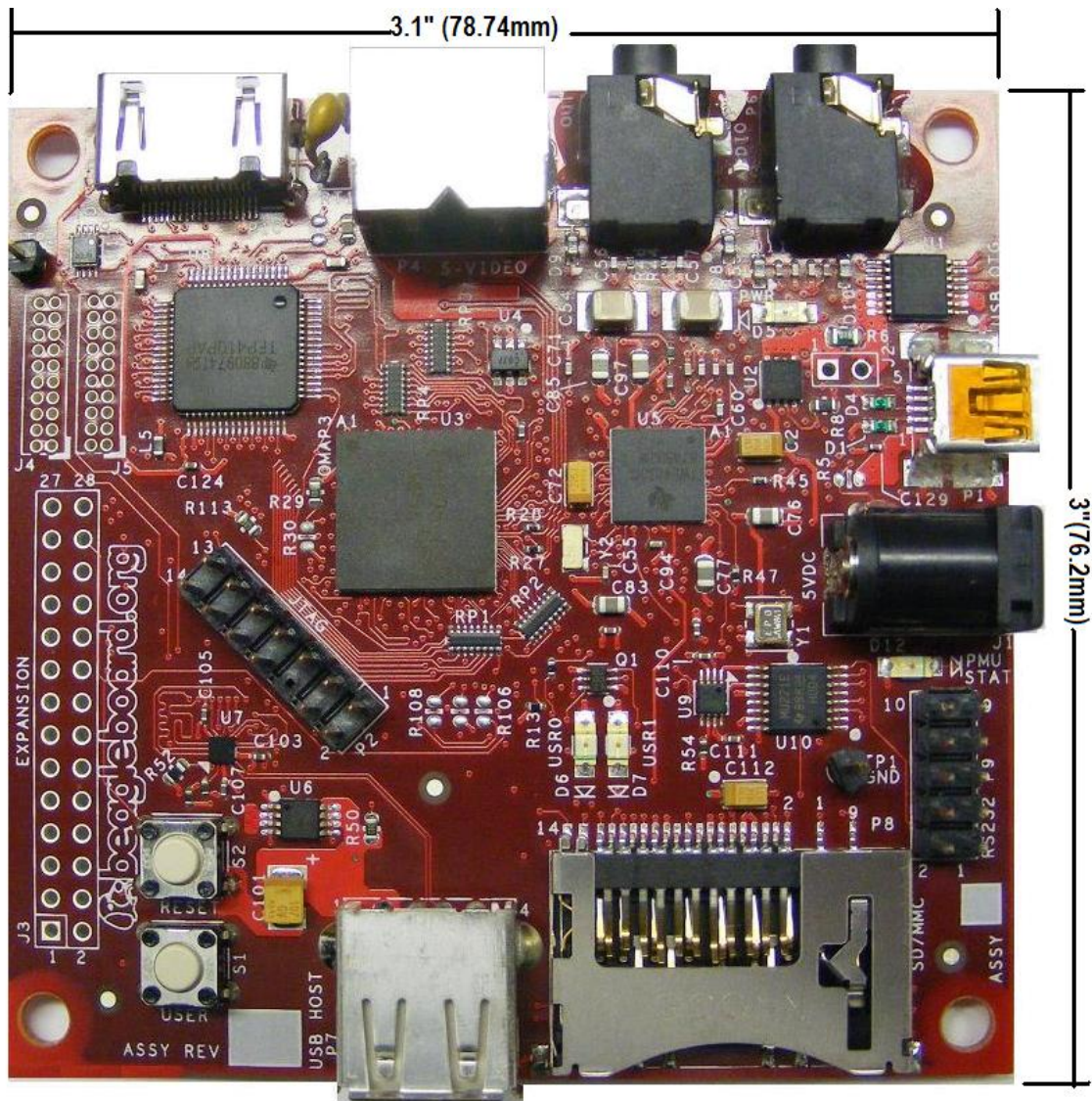
Figure 73. BeagleBoard Dimension Drawing
