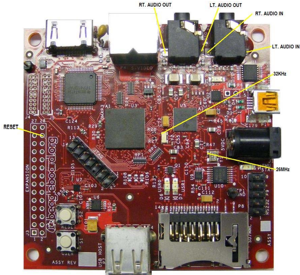
Figure 80. BeagleBoard Signal Access Points
