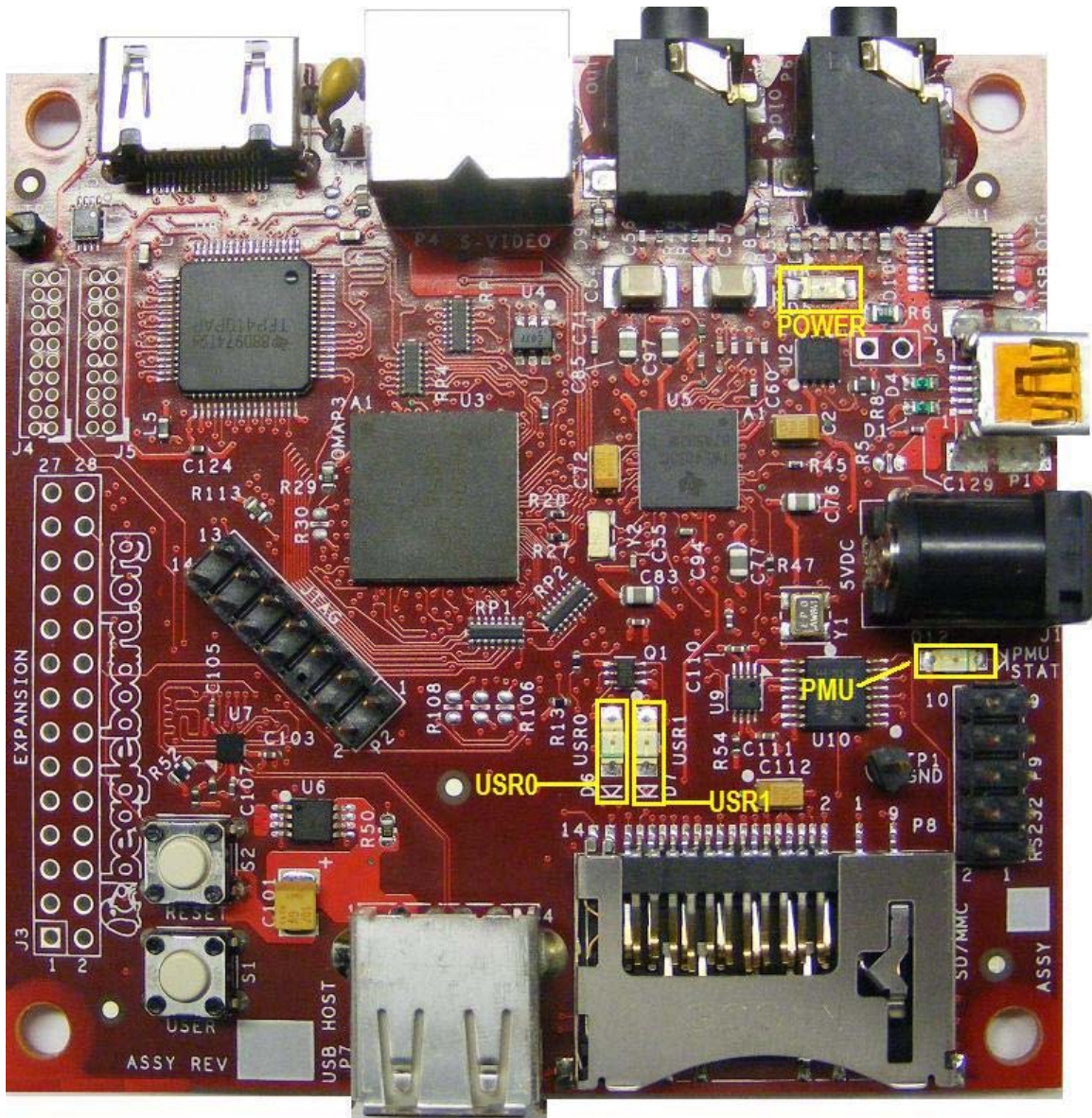
Figure 14. BeagleBoard Indicator Locations
