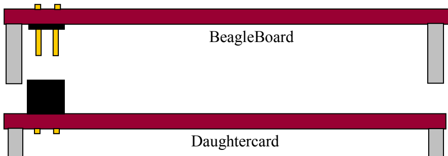
Figure 75. BeagleBoard Bottom Stacked Daughter Card
