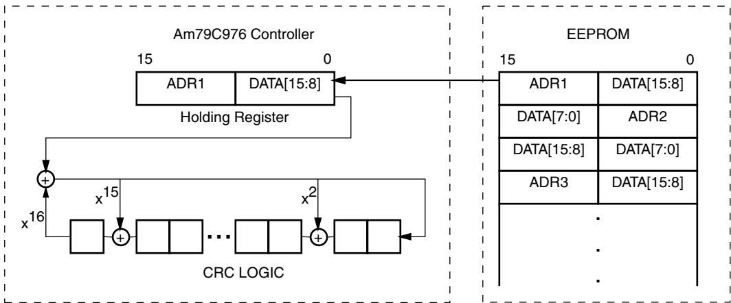
Figure 42. CRC Flow
