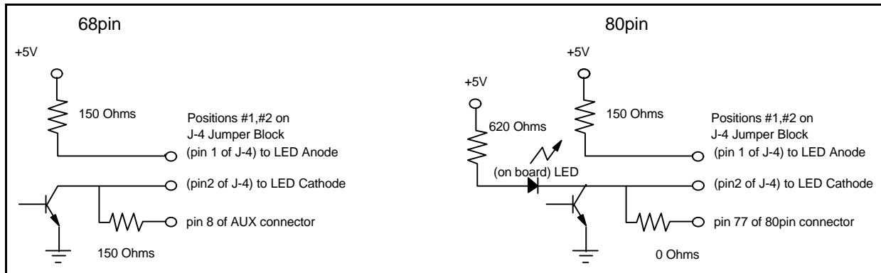
Figure 24. LED circuit
