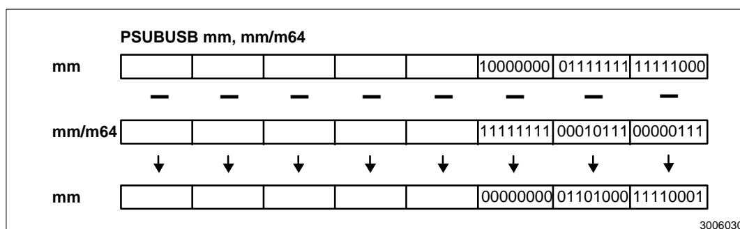
Figure 2-21. Operation of the PSUBUSB Instruction
