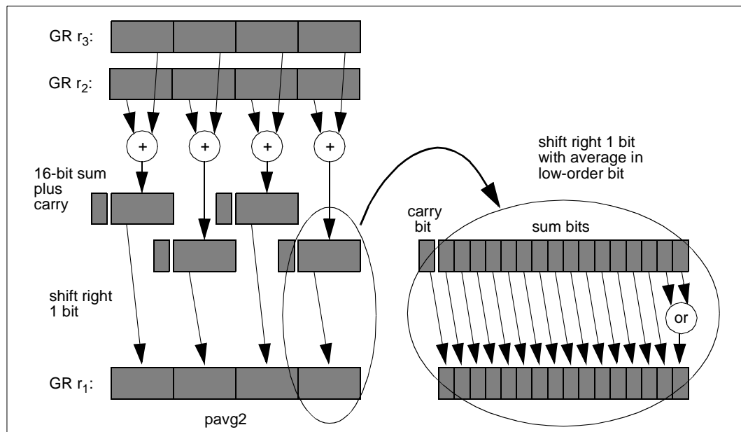
Figure 2-30. Parallel Average Example
