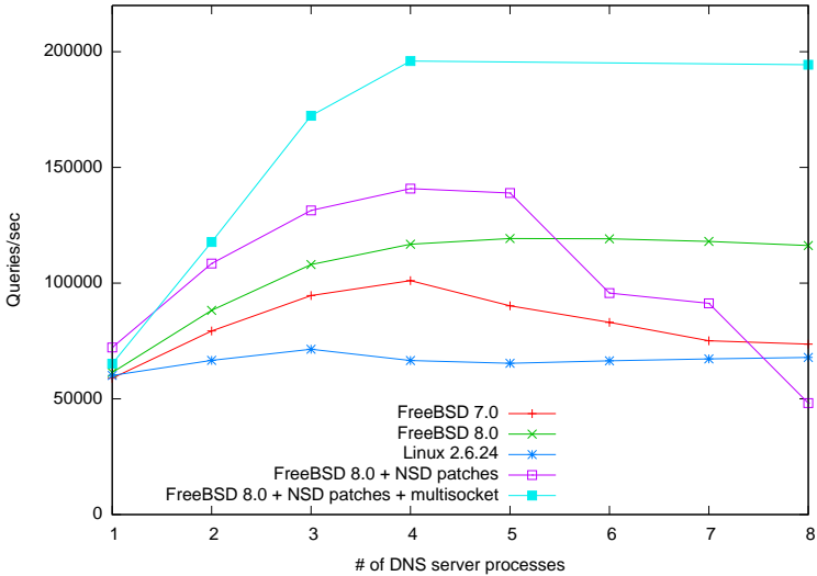
nsd 3.0.7 on 8-core xeon (10 gigabit ethernet)
