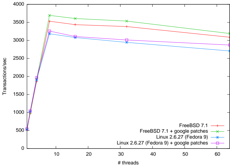
MySQL sysbench read-only performance on 8-core Xeon
