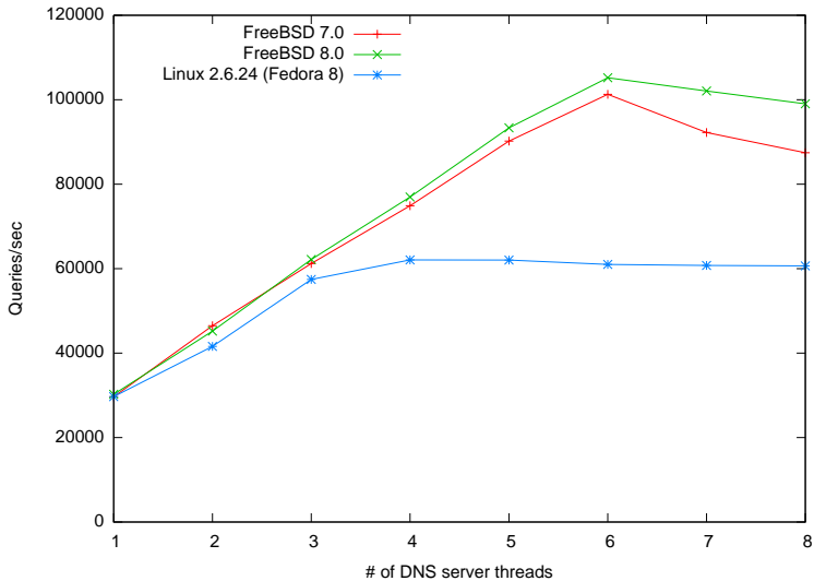
BIND 9.4.2 on 8-core xeon (10 gigabit ethernet, .pt zone)
