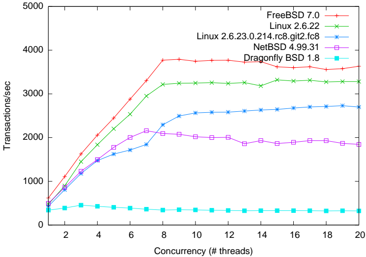
MySQL sysbench on 8-core xeon
